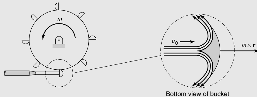
Figure 5.12 Pelton wheel.
