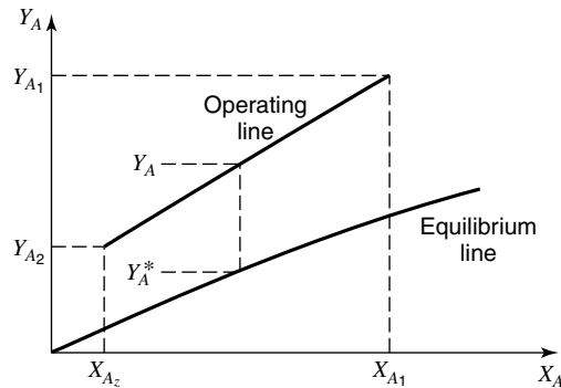
Figure 31.17 Evaluation of Y_A - Y_A^* the overall driving force.
