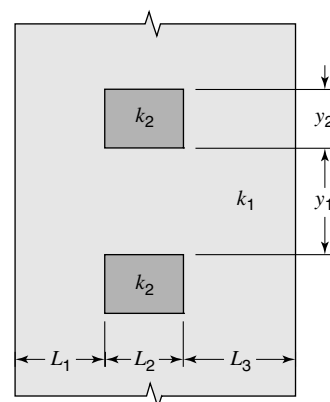
Figure 17.3 A series-parallel composite wall.
