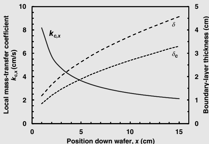
Figure 28.7 Local mass-transfer coefficient vs. position along the wafer in the direction of the gas stream, Example 3.
