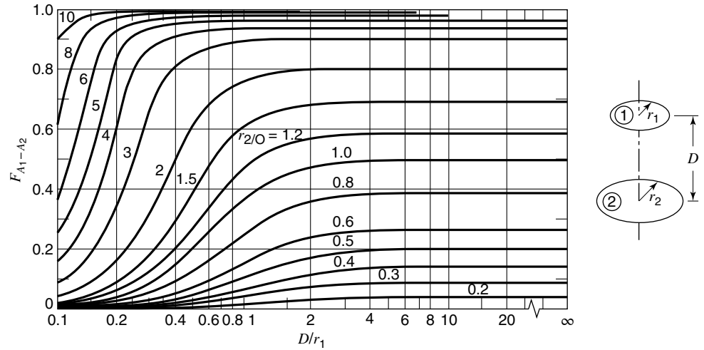
Figure 23.16 View factors for parallel opposed circular disks of unequal size.
