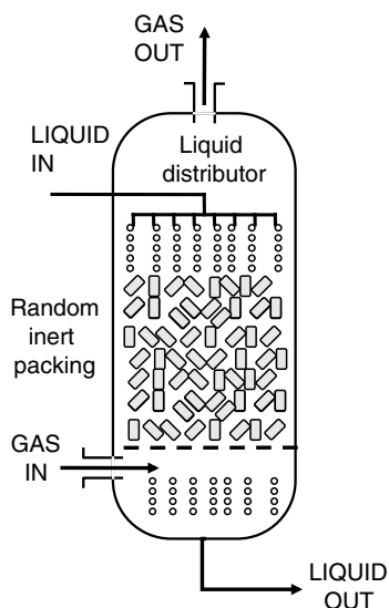
Figure 30.8 Countercurrent flow gas-liquid packed tower.
