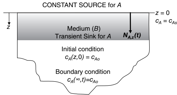
Figure 27.1 Transient diffusion in a semi-infinite medium.
