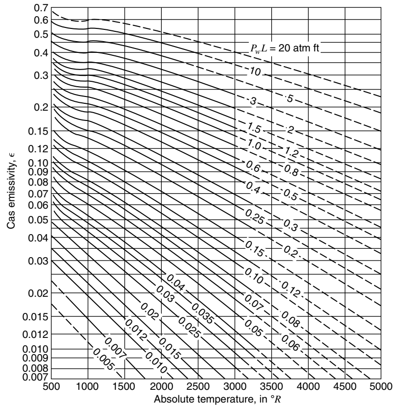
Figure 23.24 Emissivity of water vapor at one atmosphere total pressure and near-zero partial pressure.
