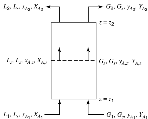
Figure 31.13 Steady-state cocurrent process.
