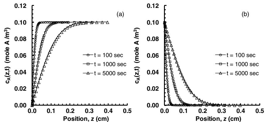
Figure 27.2 Representative concentration profiles for transient diffusion of species (A) in semi-infinite medium (B) with diffusion coefficient D_{AB} = 1.0 \times 10^{-6} \text{ cm}^2/\text{s} . (a) Medium is a source for transfer of A with c_{A0} = 0.10 \text{ mole/m}^3 and c_{As} = 0 . (b) Medium is a sink for transfer of A, with c_{A0} = 0 , and c_{As} = 0.10 \text{ mole/m}^3 .
