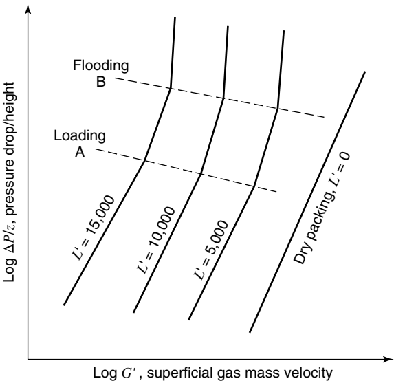
Figure 31.22 Typical gas pressure drop for countercurrent, packed tower.
