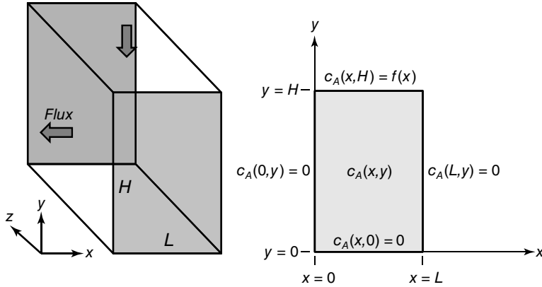
Figure 26.13 Two-dimensional diffusion.
