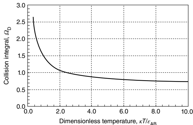
Figure 24.3 Lennard–Jones “collision integral” for diffusion as a function of dimensionless temperature.
