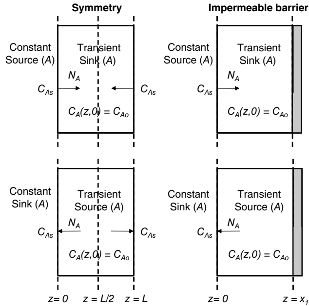
Figure 27.4 Transient diffusion in finite-dimensional medium, comparing transient source for A vs. transient sink for A.
