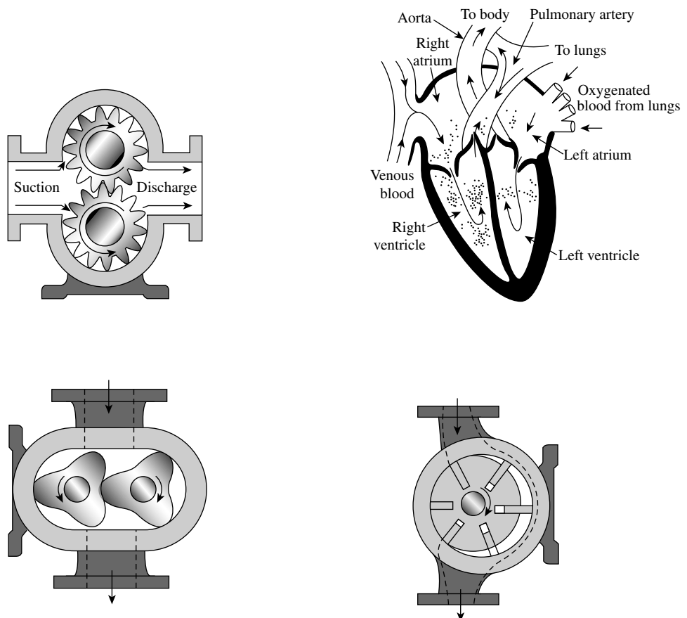
Figure 14.1 Some examples of positive-displacement configurations.
