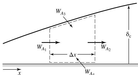
Figure 28.8 The concentration boundary-layer control volume.
