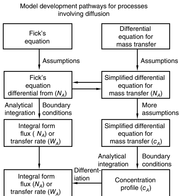
Figure 25.4 Model development pathways for processes involving molecular diffusion.
