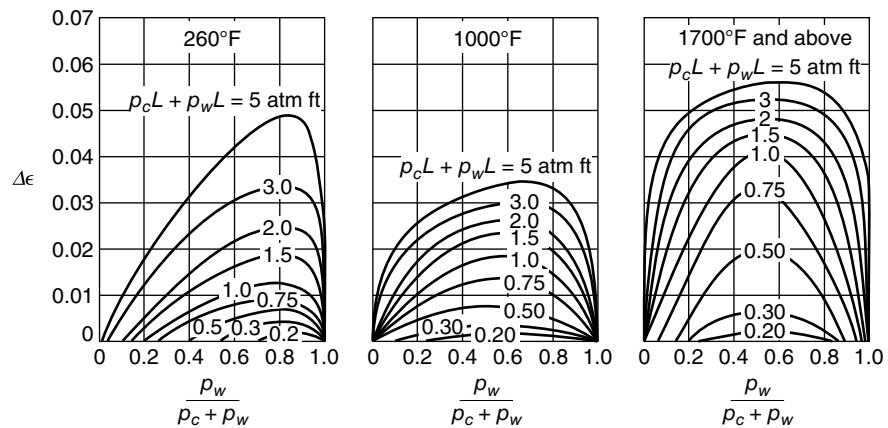
Figure 23.28 Correction to gas emissivity due to spectral overlap of \text{H}_2\text{O} and \text{CO}_2 .
