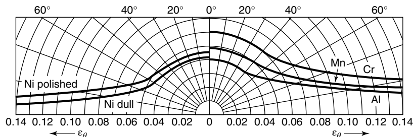
Figure 23.10 Emissivity variation with direction for conductors.
