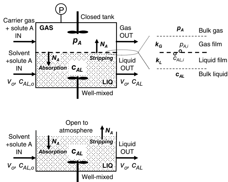
Figure 29.10 Steady-state, well-mixed, gas–liquid mass-transfer process across a defined interface.
