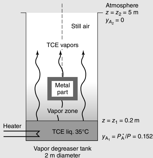
Figure 26.4 TCE emissions from a vapor degreaser.
