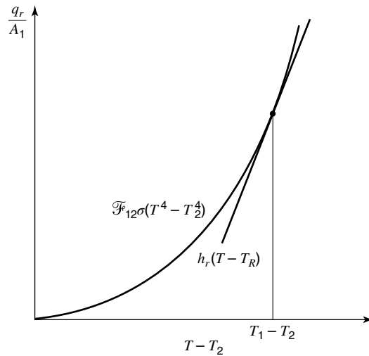
Figure 23.29 Tangent approximation for h_r .
