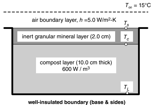
Cross section of compost bed.
