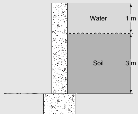
Figure 2.7 Retaining wall.
