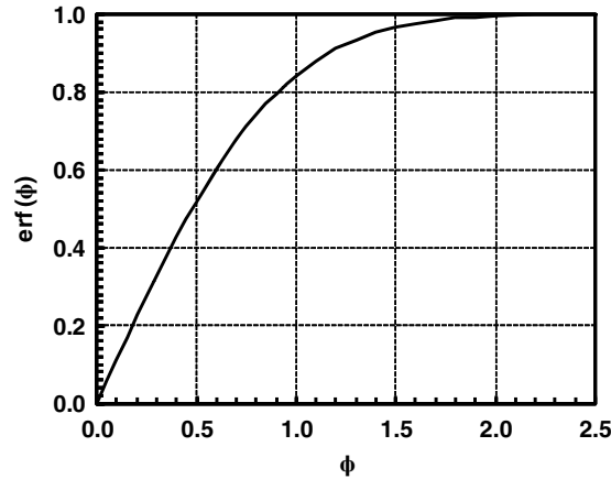
Figure 27.3 Error function.
