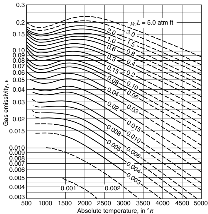
Figure 23.26 Emissivity of \text{CO}_2 at one atmosphere total pressure and near-zero partial pressure.
