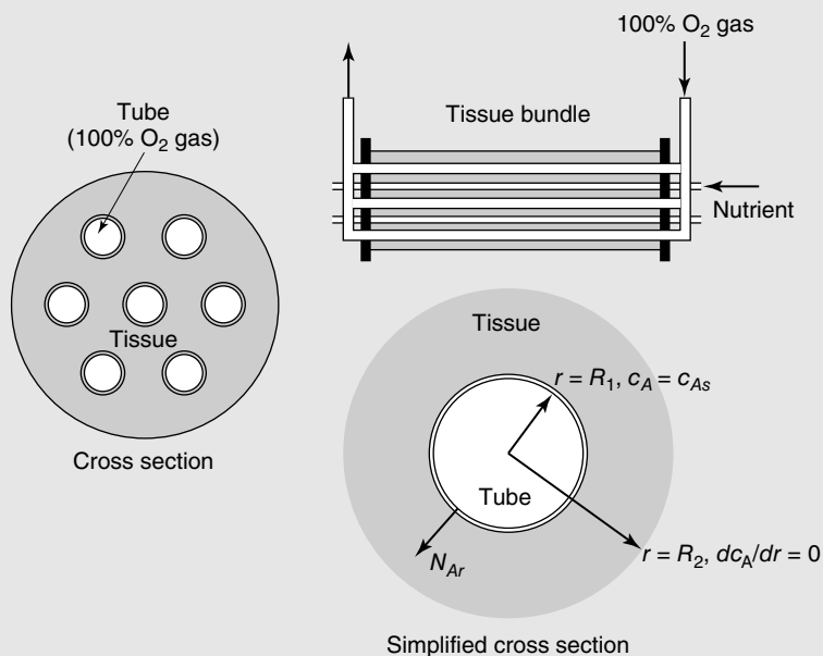
Figure 25.8 Oxygen transport within an engineered tissue bundle.
