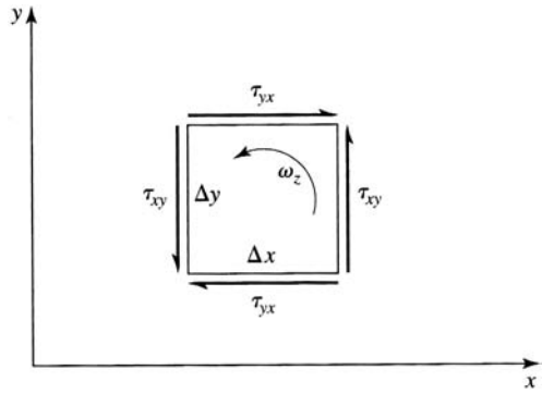
Figure C.1 Free body of element
