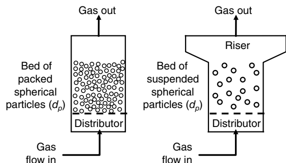
Figure 30.5 Packed vs. fluidized bed.
