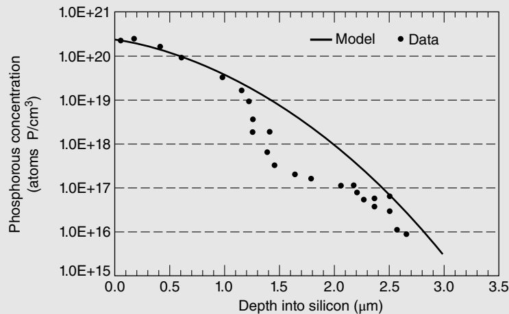
Figure 27.6 Phosphorous doping profile in silicon wafer after 1 h at 1100^\circ\text{C} .
