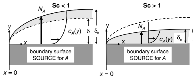
Figure 28.5 Location of concentration boundary layer ( \delta_c ) relative to hydrodynamic boundary layer ( \delta ) for \text{Sc} < 1 , and \text{Sc} > 1 .
