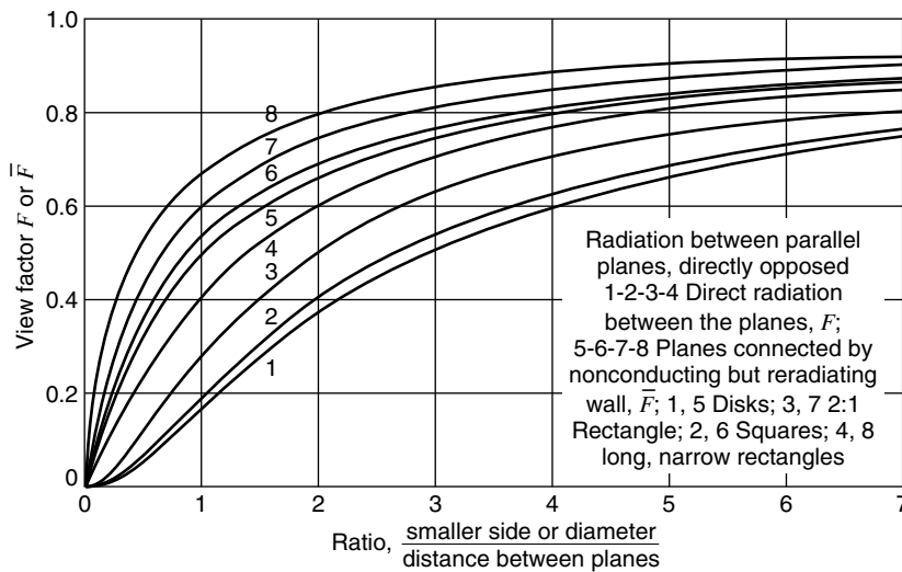
Figure 23.15 View factors for equal and parallel squares, rectangles, and disks. The curves labeled 5, 6, 7, and 8 allow for continuous variation in the sidewall temperatures from top to bottom. (From H. C. Hottel, "Radiant Heat Transmission," Mech. Engrg. , 52 (1930). By permission of the publishers.)
