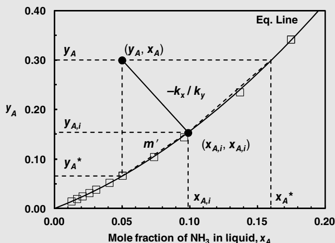
Figure 29.9 Graphical representation of gas-liquid interphase mass-transfer process for transfer of ammonia ( \text{NH}_3 ) from a gas mixture to water, Example 2.
