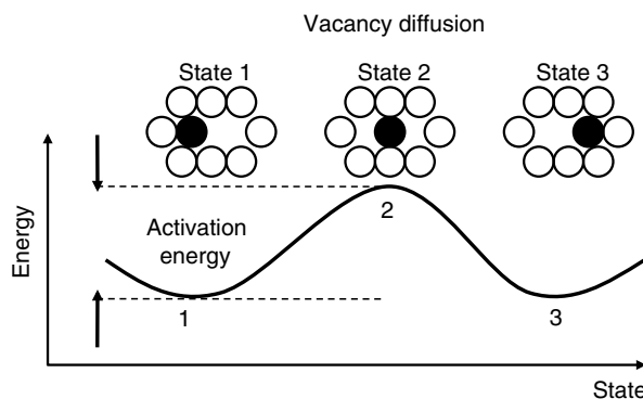
Figure 24.10 Solid-state vacancy diffusion.
