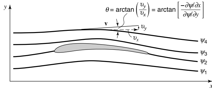
Figure 10.2 Streamlines and the stream function.
