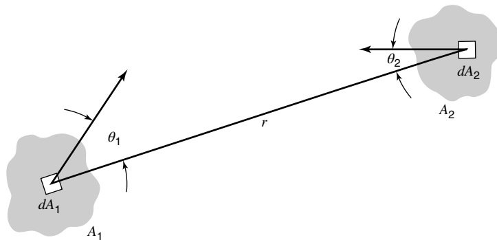
Figure 23.11 Radiant heat transfer between two surfaces.
