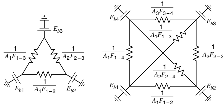
Figure 23.17 Radiation analogs.
