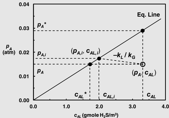
Figure 29.8 Graphical representation of gas-liquid interphase mass-transfer process for transfer of hydrogen sulfide ( \text{H}_2\text{S} ) dissolved in water into air, Example 1.
