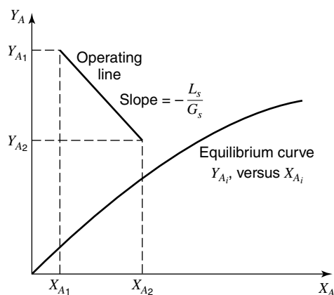
Figure 31.14 Steady-state cocurrent process, transfer from phase G to phase L .
