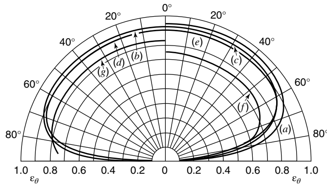
Figure 23.9 Emissivity variation with direction for nonconductors. (a) Wet ice. (b) Wood. (c) Glass. (d) Paper. (e) Clay. (f) Copper oxide. (g) Aluminum oxide.
