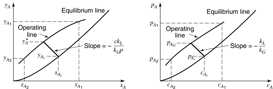
Figure 31.19 Determination of interfacial composition for transfer from phase G to phase L .
