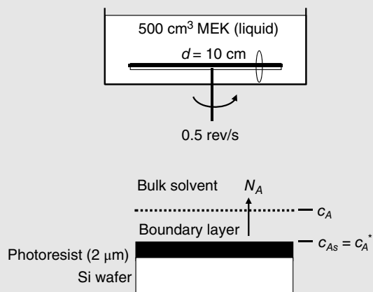
Figure 30.11 Dissolution of photoresist coating on spinning silicon wafer disk into methyl ethyl ketone (MEK) solvent.
