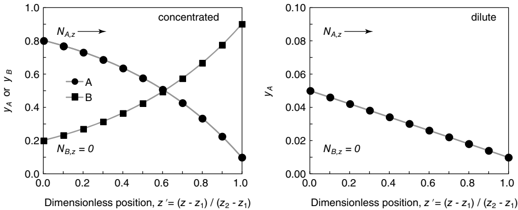
Figure 26.3 Concentration profiles for unimolecular diffusion of component A in concentrated and dilute systems.
