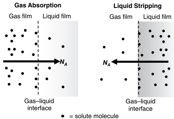
Figure 29.3 Gas absorption vs. liquid stripping for transfer of solute A between contacting gas and liquid phases.
