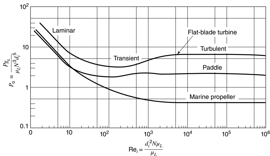
Figure 30.7 Power number vs. Reynolds number for impellers immersed in single-phase liquids. 22
