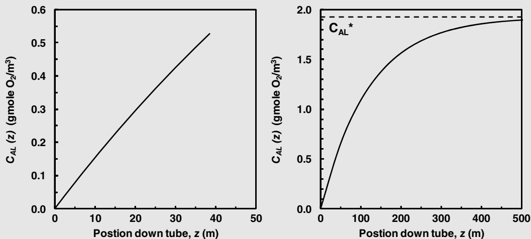
Figure 30.14 Dissolved oxygen profile in bubbleless membrane for aeration of water.
