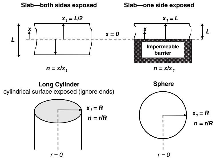
Figure 27.10 One-dimensional diffusion geometries for concentration-time charts.
