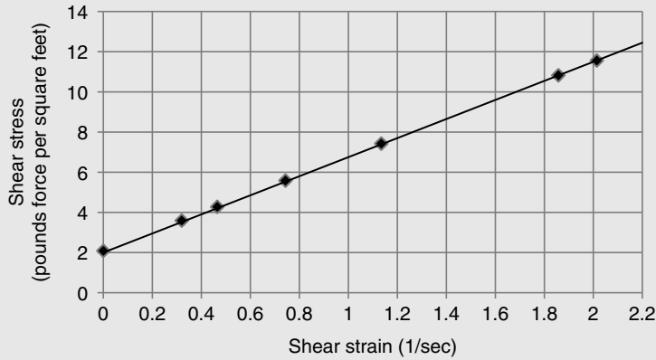
Figure 7.9 Shear stress versus shear strain for mayonnaise.
