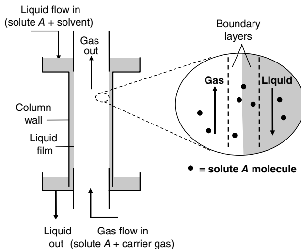
Figure 29.1 Wetted wall tower for transfer of solute A between contacting gas and liquid phases.
