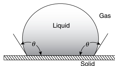
Figure 1.8 Contact angle for a non-wetting gas-liquid-solid interface.
