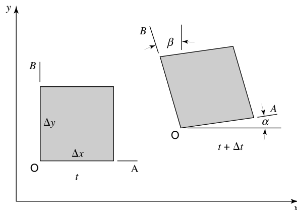
Figure 10.1a Rotation of a fluid element.
