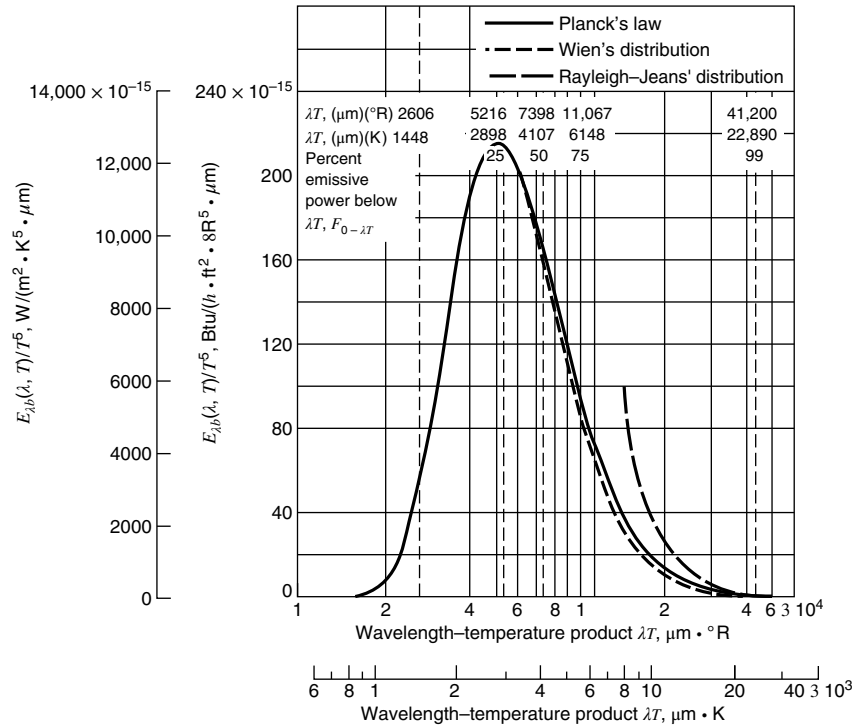
Figure 23.6 Spectral energy distribution for a black body as a function of \lambda T . (From R. Siegel and J. R. Howell, Thermal Radiation Heat Transfer , 3rd edition, Hemisphere Publishers, Washington, 1992. By permission of the publishers.)
