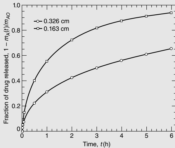
Figure 27.8 Fractional drug release vs. time profiles.
