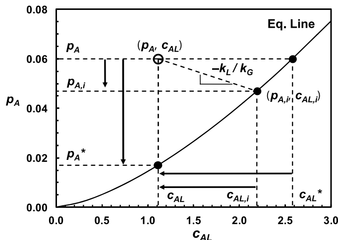
Figure 29.6 Graphical representation of gas–liquid interphase mass-transfer process for gas absorption.
