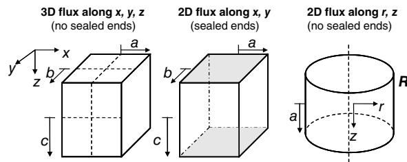
Figure 27.11 Two- and three-dimensional diffusion geometries for concentration-time charts.
