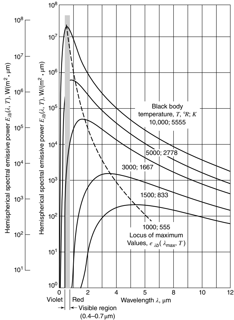
Figure 23.5 Spectral emissive power for a black body for several temperatures. (From R. Siegel and J. R. Howell, Thermal Radiation Heat Transfer , 3rd edition, Hemisphere Publishers, Washington, 1992. By permission of the publishers.)
