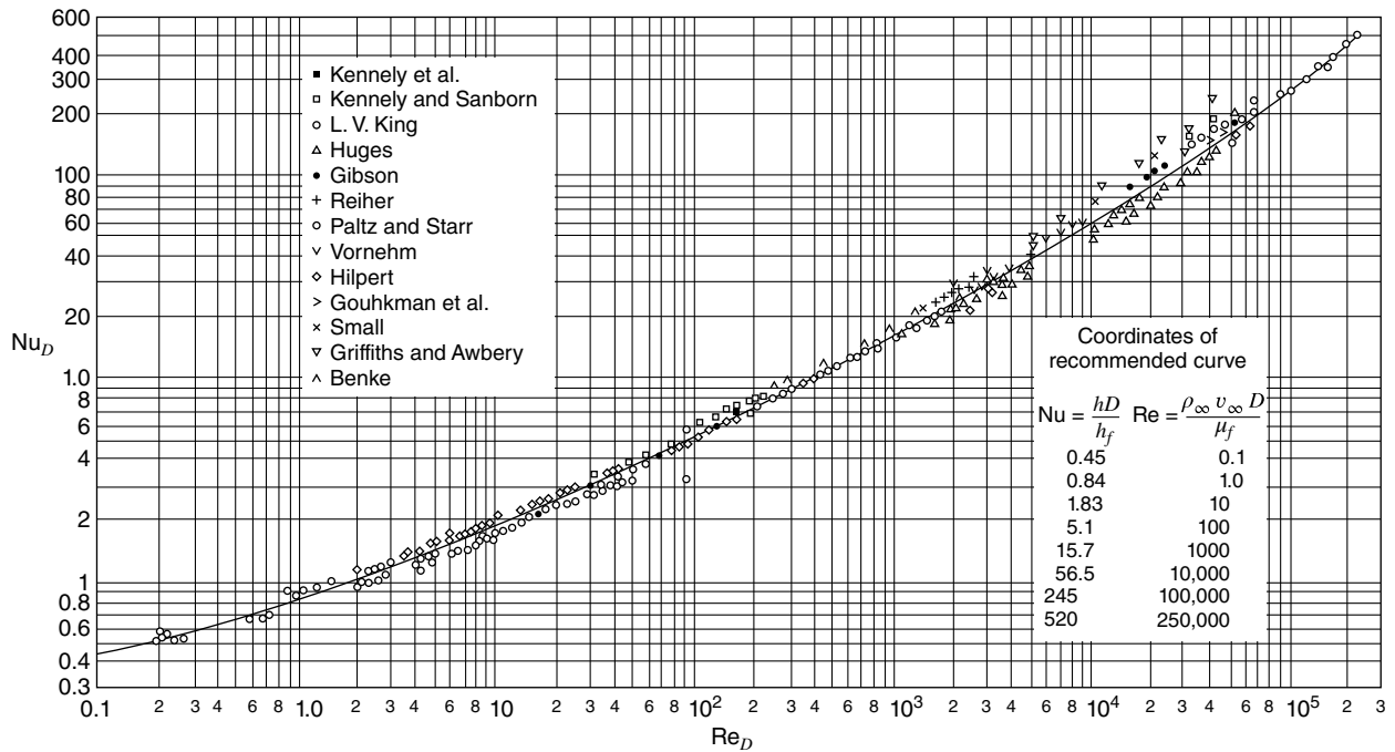
Figure 20.9 Nu vs. Re for flow normal to single cylinders. Note: These values are strictly valid when Pr \approx 1 . (From W. H. McAdams, Heat Transmission , 3rd edition, McGraw-Hill Book Company, New York, 1954, p. 259.)
