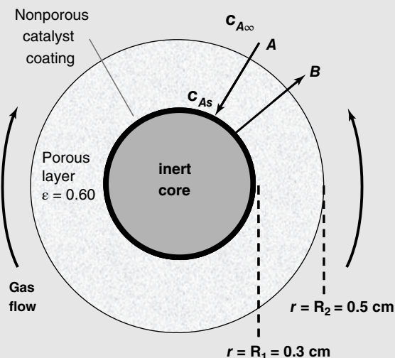
Figure 26.9 Cross section of catalyst particles for Example 3.
