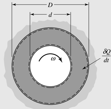
Figure 6.7 Bearing and control volume for bearing analysis.
