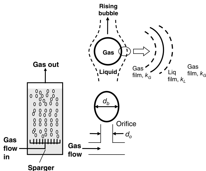
Figure 30.2 Gas bubbles dispersed in liquid column.
