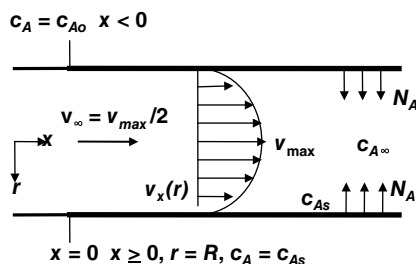
Figure 30.3 Laminar flow mass transfer within a pipe.
