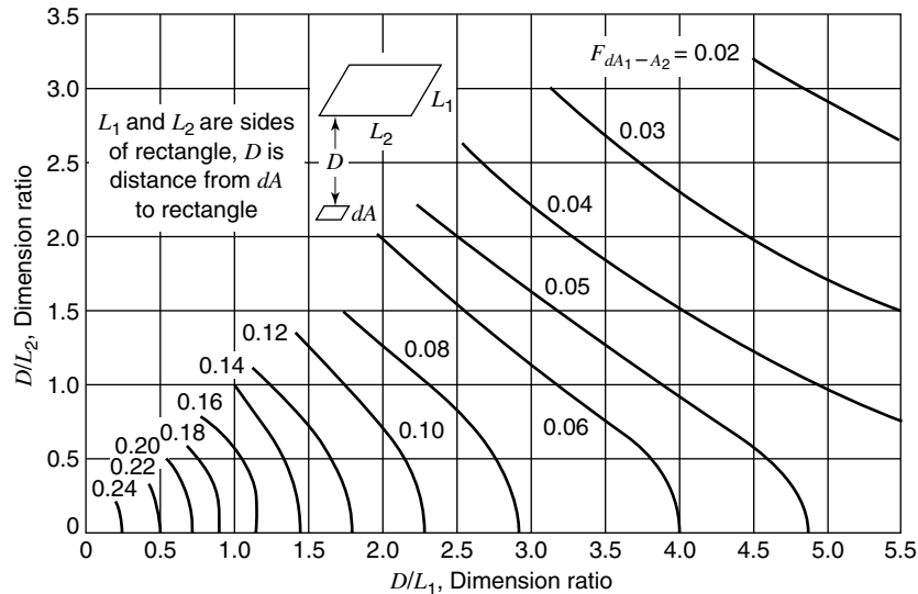
Figure 23.13 View factor for a surface element and a rectangular surface parallel to it. (From H. C. Hottel, “Radiant Heat Transmission,” Mech. Engrg. , 52 (1930). By permission of the publishers.)
