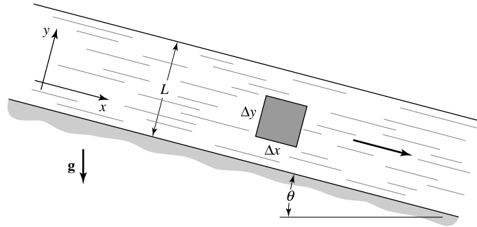
Figure 8.2 Laminar flow down an inclined-plane surface.
