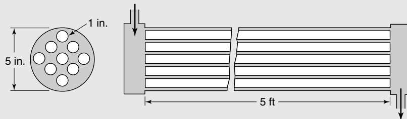
Figure 13.3 Shell-and-tube head-exchanger configuration.
