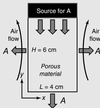
Figure 26.14 Mass-transfer system for Example 5.
