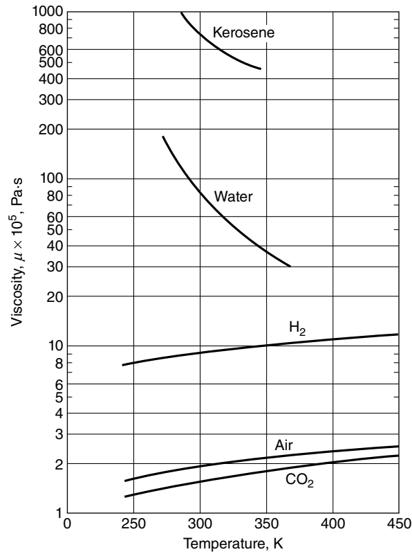
Figure 7.5 Viscosity–temperature variation for some liquids and gases.
