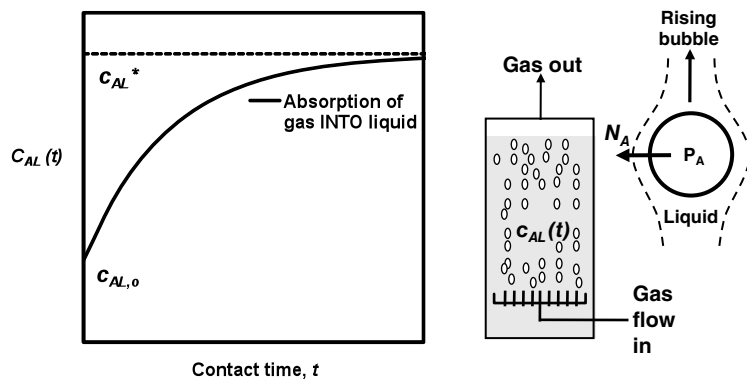
Figure 30.9 Example of well-mixed, unsteady-state mass-transfer process: absorption of bubbled gas into a tank of liquid.
