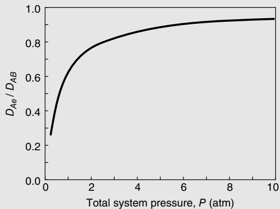
Figure 24.6 Effect of total system pressure on the ratio of the effective diffusion coefficient to the binary gas-phase molecular diffusion coefficient, Example 5.
