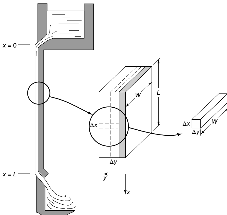
Figure 26.17 Absorption into a falling-liquid film.
