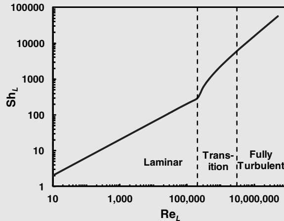
Figure 28.9 Average Sherwood number ( \text{Sh}_L ) at \text{Sc} = 1.0 for flow over a flat plate, showing transition from laminar to fully turbulent regimes, Example 4.
