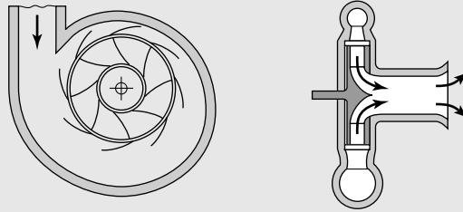
Figure 5.15 Radial-flow turbine.
