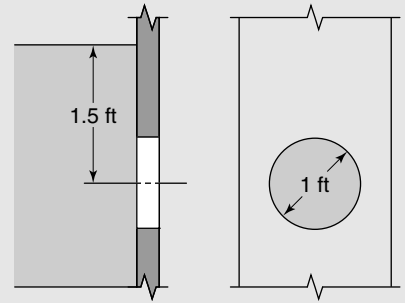
Figure 2.6 Submerged window.
