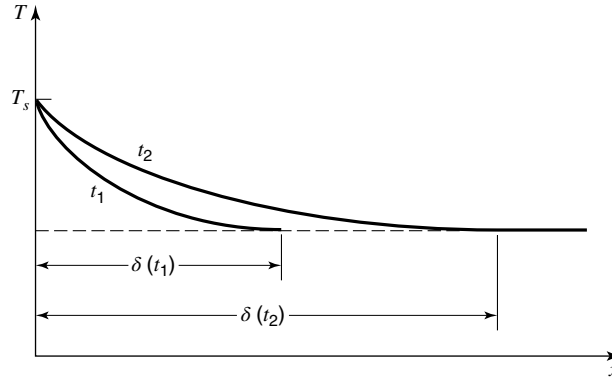
Figure 18.6 Temperature profiles at two times after the surface temperature is raised to T_s .
