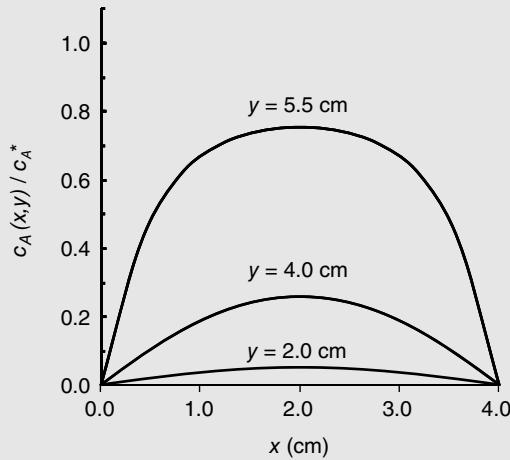
Figure 26.15 Normalized two-dimensional concentration profiles for Example 5.
