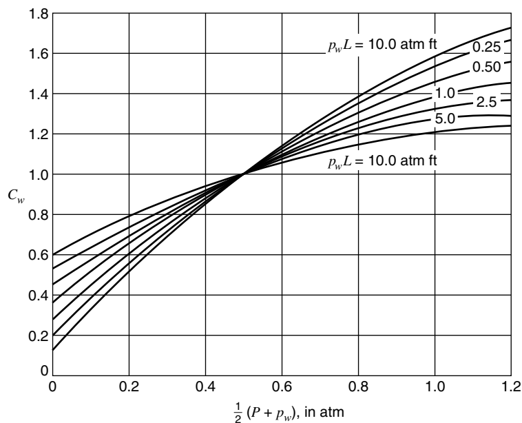
Figure 23.25 Correction factor for converting emissivity of \text{H}_2\text{O} at one atmosphere total pressure to emissivity at P atmospheres total pressure.
