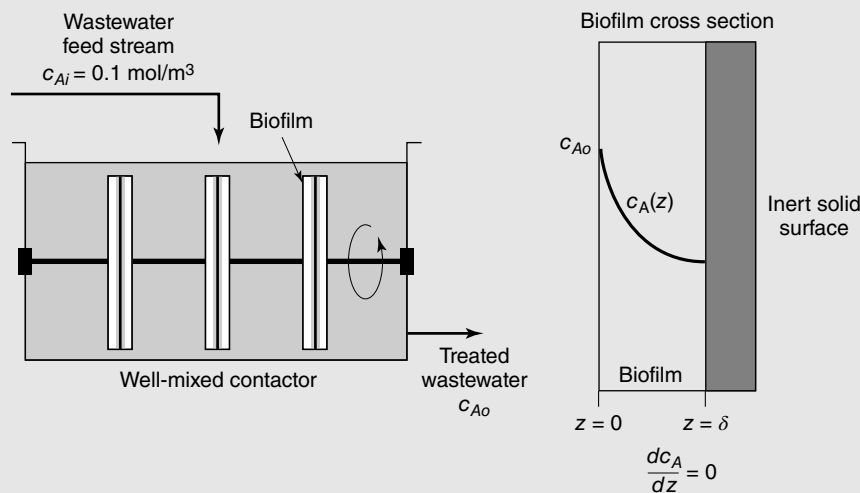
Figure 26.11 Biofilm for wastewater treatment.
