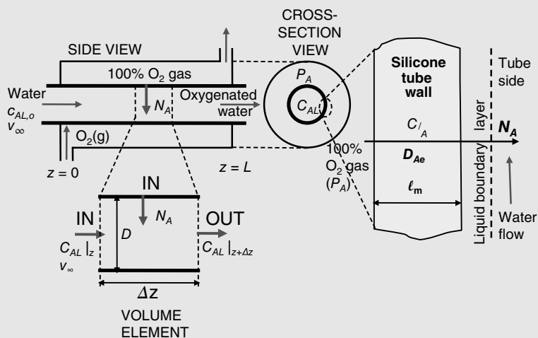
Figure 30.13 Bubbleless shell-and-tube membrane mass-transfer system for aeration of water.
