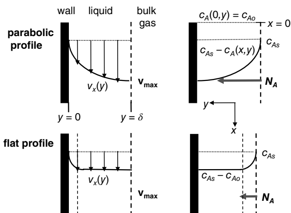
Figure 28.14 Mass transfer into falling liquid film.
