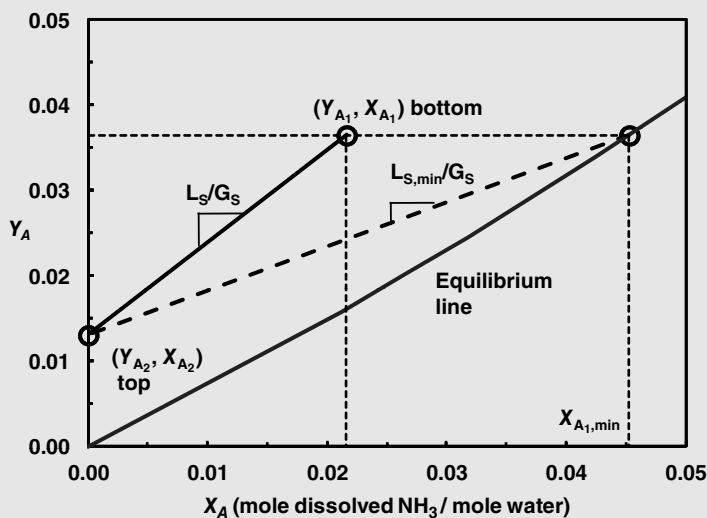
Figure 31.12 Operating and equilibrium lines for Example 3. Equilibrium distribution data from Perry and Chilton. 2
