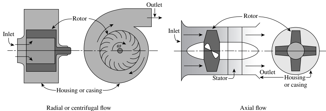
Figure 14.2 Turbomachines.
