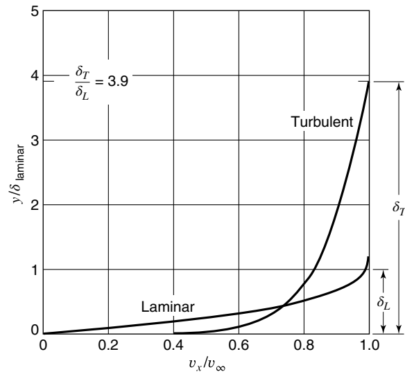
Figure 12.16 Comparison of velocity profiles in laminar and turbulent boundary layers. The Reynolds number is 500,000.
