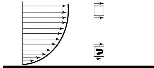
Figure 10.1b Rotation of a fluid element as the result of a velocity gradient.
