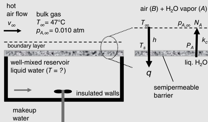
Figure 28.12 Transpiration cooling process for chilling water, Example 5.
