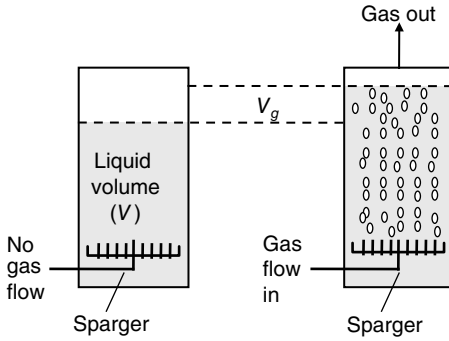
Figure 30.6 Gas holdup in bubble column.
