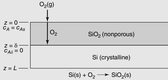
Figure 26.6 Thermal oxidation of a silicon wafer.
