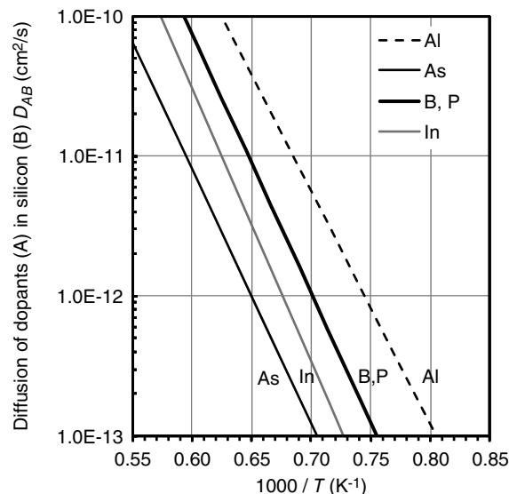
Figure 24.12 Average diffusion coefficients of substitutional dopants in polycrystalline silicon, using data provided by Gandhi. 23
