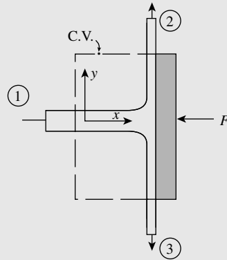
Figure 5.10 Control volume for Example 3.
