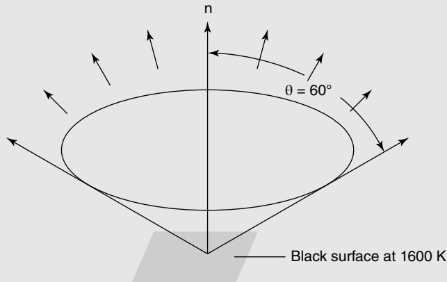
Figure 23.7 Black surface at 1600 K.
