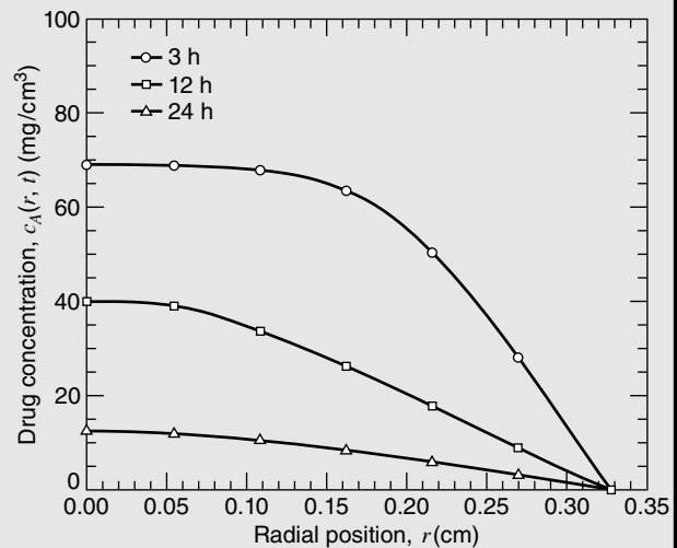
Figure 27.9 Concentration profile of a 0.326 cm radius bead after 3, 12, and 24 h.
