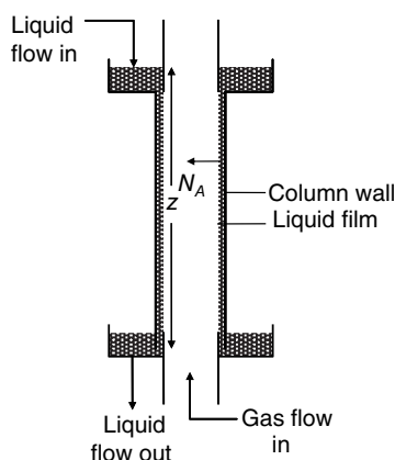
Figure 30.4 Wetted-wall column for interphase mass transfer of gas and liquid.
