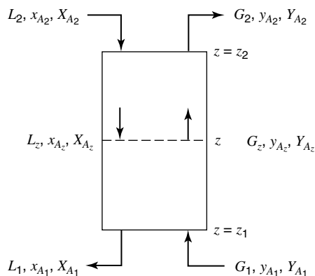
Figure 31.16 Steady-state countercurrent process.
