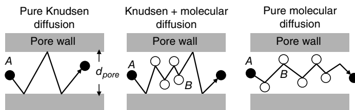
Figure 24.4 Influence of Knudsen and molecular diffusion on the effective diffusion within a straight pore.
