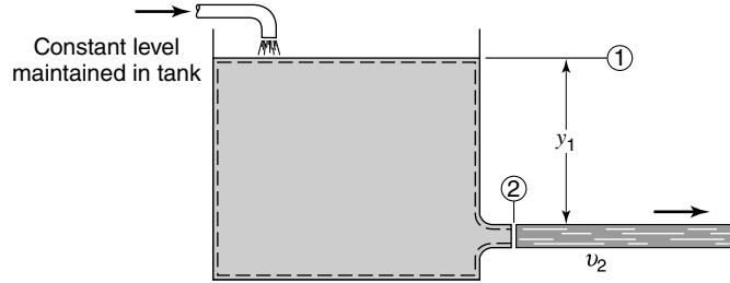
Figure 6.9 Control volume for Bernoulli equation analysis.
