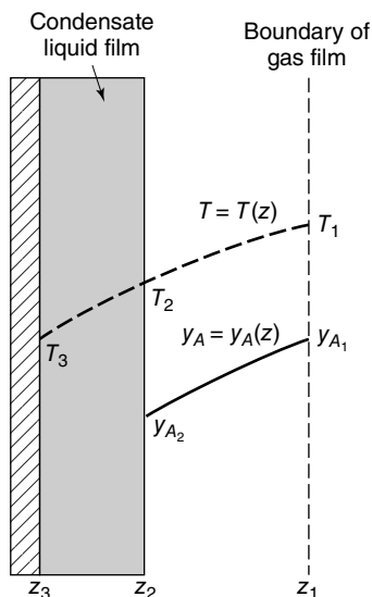
Figure 26.16 Vapor condensation on a cold surface.
