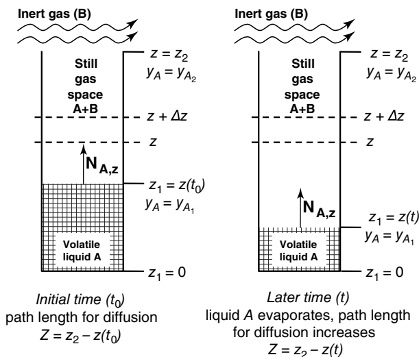
Figure 26.5 Arnold diffusion cell with moving liquid surface.
