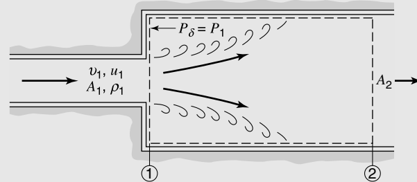
Figure 6.10 Flow through a sudden enlargement.
