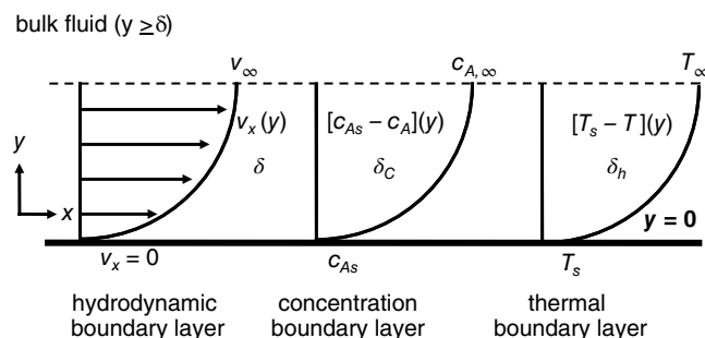
Figure 28.10 Representation of hydrodynamic, concentration, and thermal boundary layers for Sc = Pr = 1.0 associated with the Reynolds analogy.
