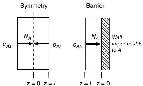
Figure 25.3 Examples of boundary conditions at z = 0 where the net flux is zero.
