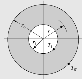
Figure 15.3 Heat conduction in a radial direction with uniform surface temperatures.
