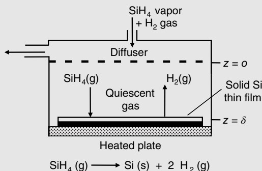
Figure 25.5 Chemical vapor deposition of a silicon thin film from silane gas.
