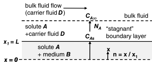
Figure 27.12 Physical situation for convection mass-transfer resistance at the boundary.
