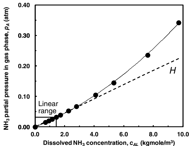
Figure 29.2 Ammonia solubility in water vs. partial pressure of ammonia at 30°C.
