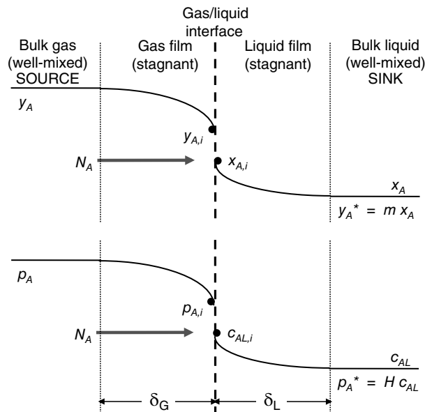
Figure 29.4 Concentration gradients between contacting gas and liquid phases where solute A is transferred from the bulk gas to the bulk liquid.
