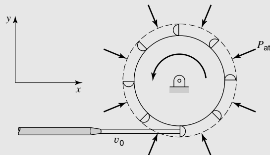
Figure 5.13 Control volume for analysis of Pelton wheel.
