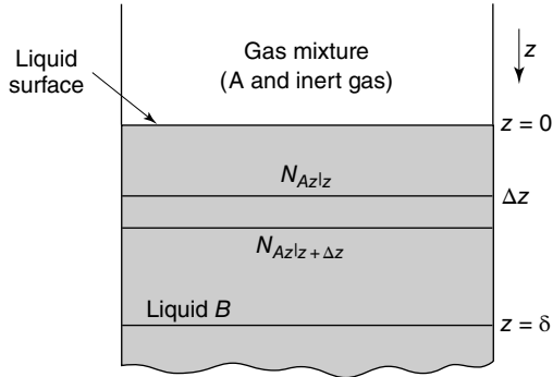
Figure 26.10 Absorption with homogeneous chemical reaction.
