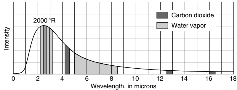
Figure 23.23 Emission bands of \text{CO}_2 and \text{H}_2\text{O} .
