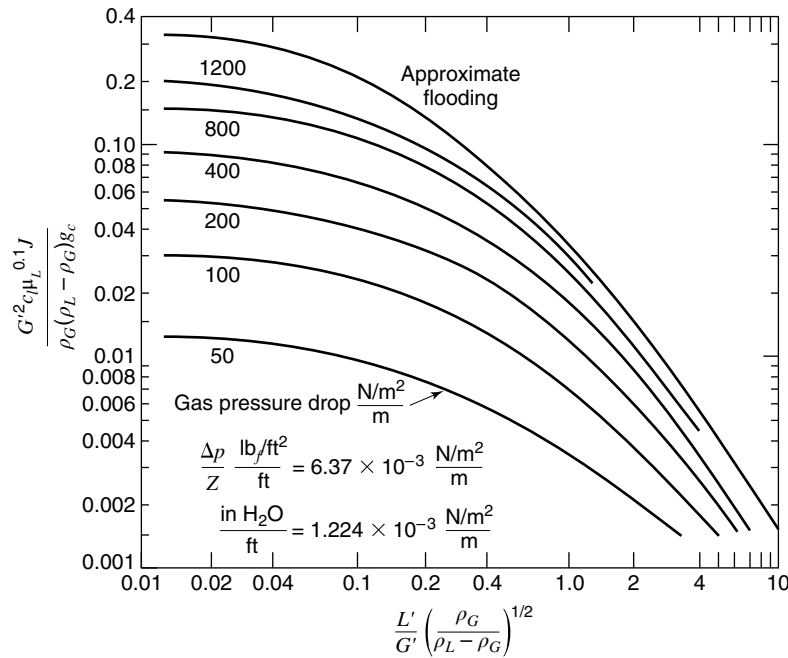
Figure 31.23 Flooding correlation for random-packed towers.
