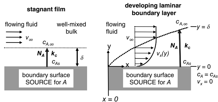
Figure 28.1 Film theory and boundary-layer theory representation of convective mass transfer for flow over a flat surface.
