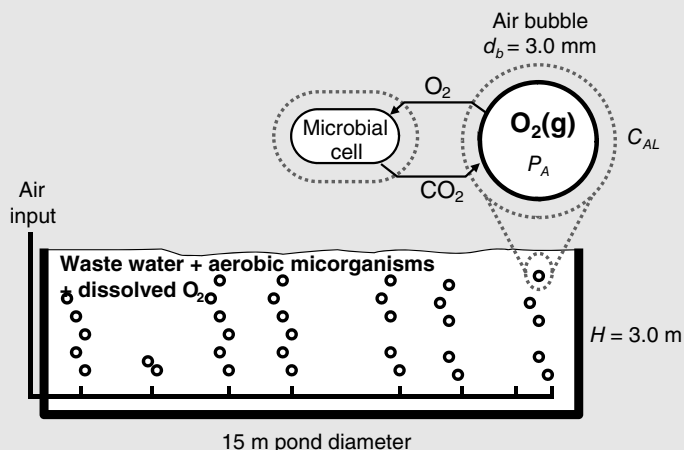
Figure 30.12 Oxygen transfer in an aerated pond containing microorganisms.
