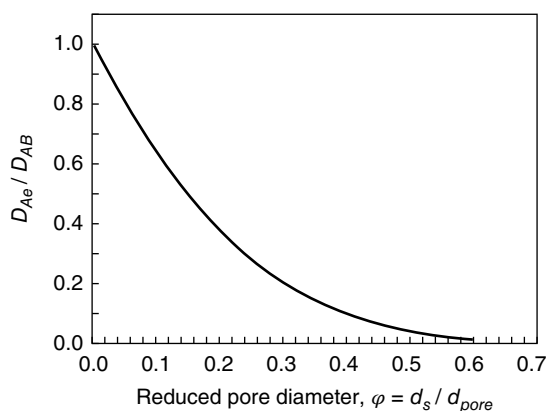
Figure 24.8 Effect of reduced pore diameter on the effective diffusion coefficient, using the Renkin equation for the hydrodynamic hindrance factor.
