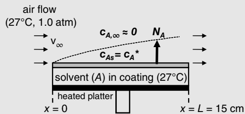
Figure 28.2 Evaporation of MEK solvent vapor from wet photoresist coating into a flowing air stream, Example 1.
