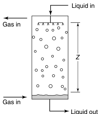
Figure 31.2 Spray tower.
