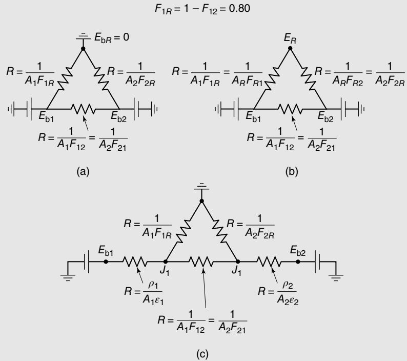
Figure 23.22 Equivalent circuits for example 6.
