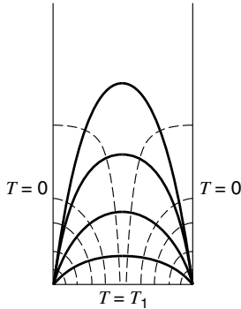
Figure 17.13 Isotherms and energy flow lines for the rectangular plate in Figure 17.12.
