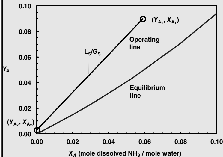
Figure 31.20 The operating line for Example 4.
