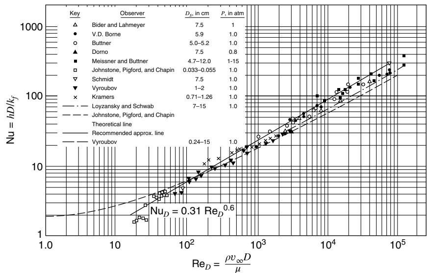
Figure 20.11 Nu_D vs. Re_D for air-flow past single spheres. (From McAdams, Heat Transmission , 3rd edition, McGraw-Hill Book Company, New York, 1954, p. 266. By permission of the publishers.)
