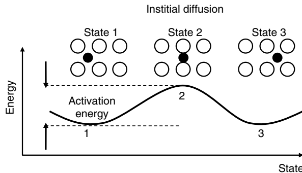
Figure 24.11 Solid-state interstitial diffusion.
