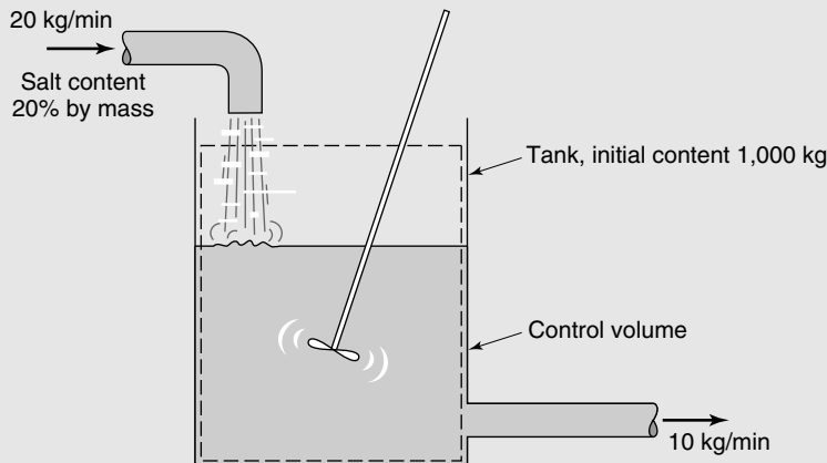
Figure 4.4 A mixing process.
