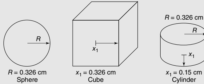
Figure 27.13 Three capsule configurations.
