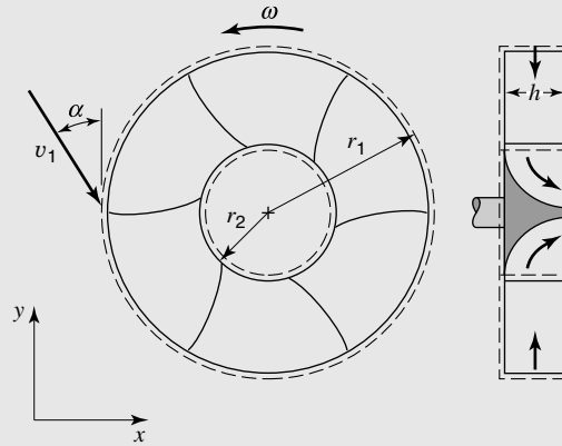
Figure 5.16 Radial-flow turbine-runner control volume.
