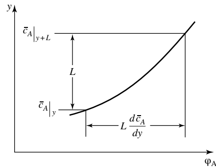
Figure 28.11 Portion of turbulent concentration profile curve, showing the Prandtl mixing length.
