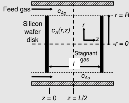
Figure 25.7 Interwafer region and control volume for Example 2.
