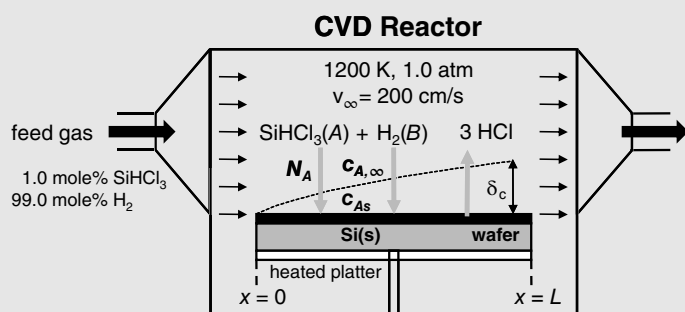
Figure 28.6 Chemical vapor deposition of solid silicon onto a wafer surface by a flowing gas stream mixture of trichlorosilane and H 2 , Example 3.
