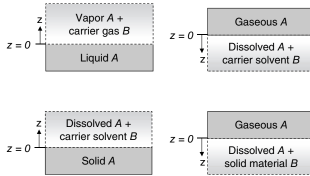
Figure 25.2 Examples of concentration boundary conditions defined by a thermodynamic equilibrium constraint at an interface.
