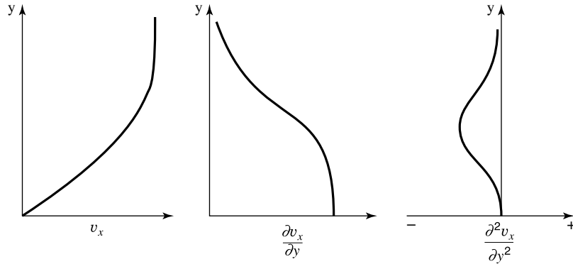
Figure 12.7 Variation in velocity and velocity derivatives across the laminar boundary layer when dP/dx = 0 .
