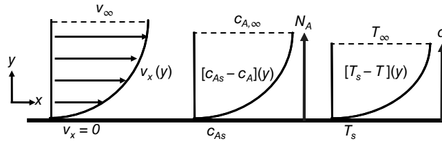
Figure 28.3 Velocity, concentration, and temperature profiles for a fluid flowing past a solid surface.
