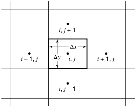
Figure 17.14 Two-dimensional volume element in a conducting medium.
