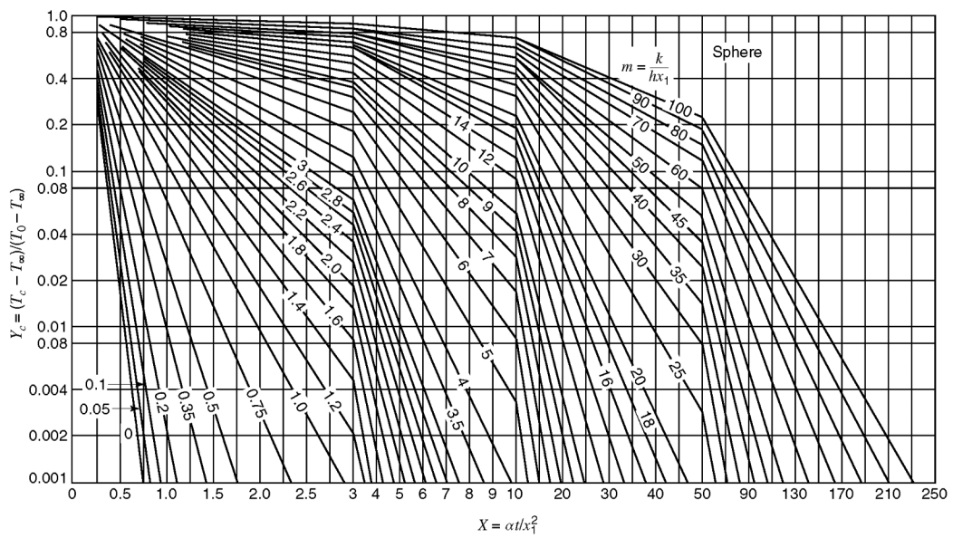
Figure F.6 Center temperature history for a sphere.
