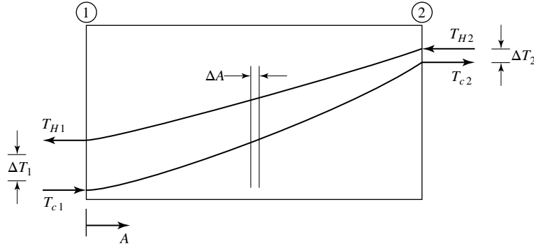
Figure 22.7 Diagram of temperature vs. contact area for single-pass counterflow analysis.
