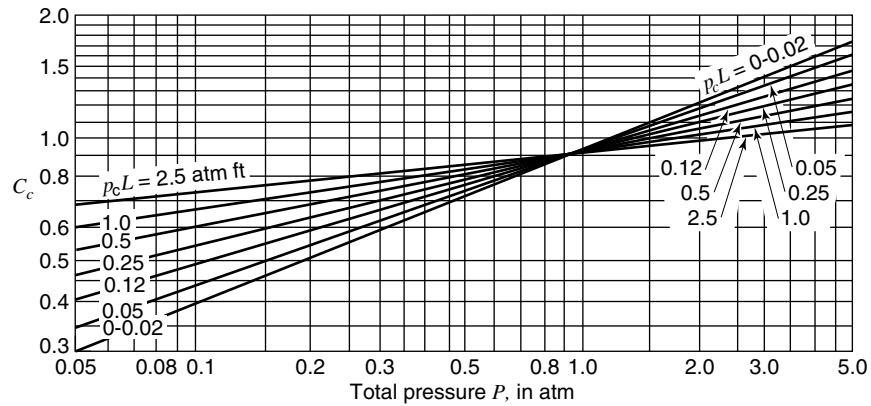
Figure 23.27 Correction factor for converting emissivity of \text{CO}_2 at one atmosphere total pressure to emissivity at P atmospheres total pressure.
