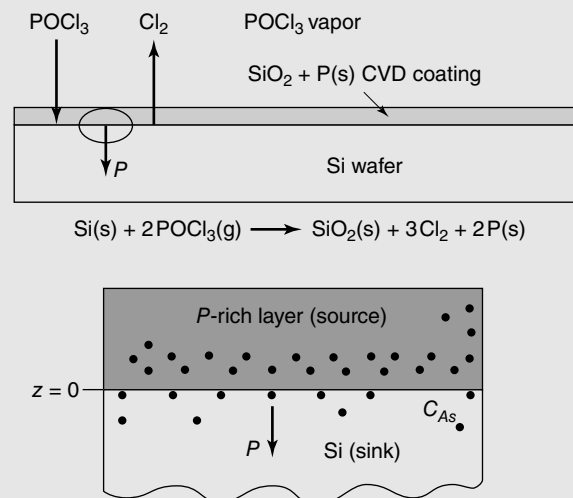
Figure 27.5 Phosphorous doping of a silicon wafer.
