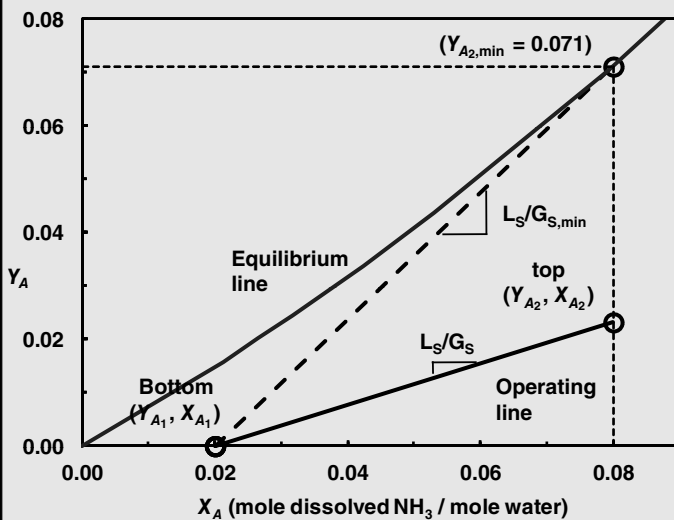
Figure 31.24 Operating and equilibrium lines for Example 7. Equilibrium distribution data from Perry and Chilton. 2
