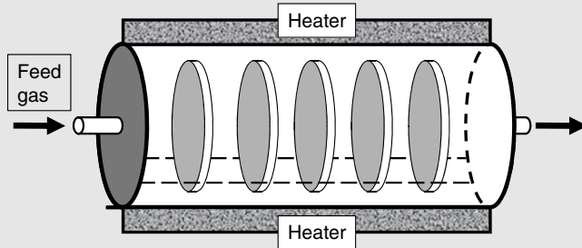
Figure 25.6 Diffusion furnace containing vertically stacked wafers.
