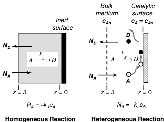
Figure 26.8 Homogeneous reaction within the control volume for diffusion vs. heterogeneous reaction at a catalytic surface.
