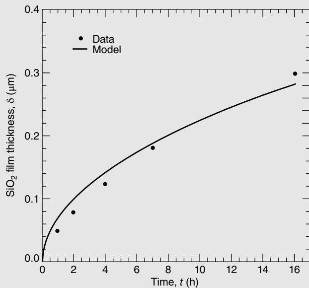
Figure 26.7 Silicon dioxide ( SiO_2 ) film thickness vs. time at 1000^\circ\text{C} .
