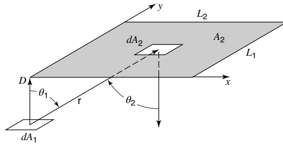
Figure 23.12 Differential area and parallel-finite area.
