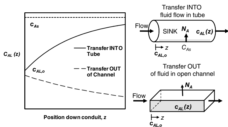
Figure 30.10 Examples of steady-state convective mass transfer where the concentration changes with position.
