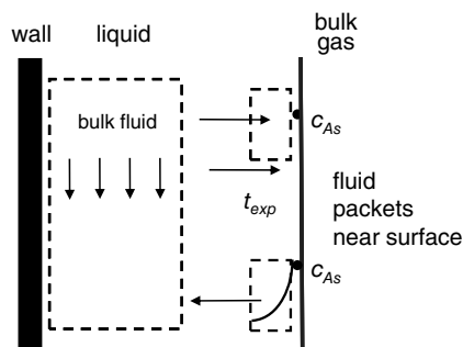
Figure 28.13 Penetration theory—surface renewal of fluid elements.
