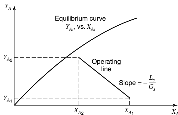
Figure 31.15 Steady-state cocurrent process transfer from phase L to phase G .
