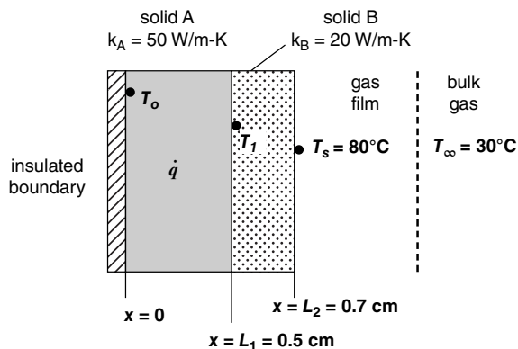
Heat transfer in composite solid.
