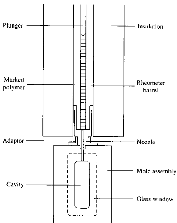
FIGURE 15.19 Injection-molding apparatus. (From Ref. 28.)
