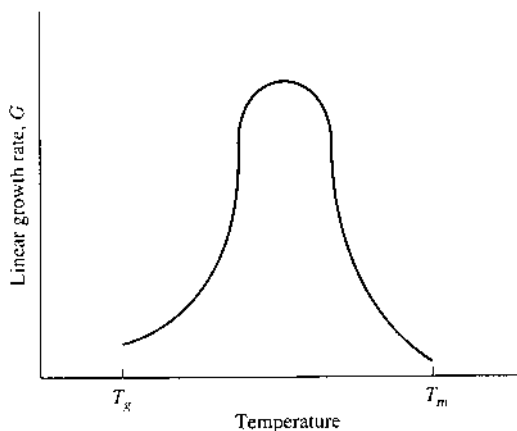
FIGURE 11.9 Qualitative temperature dependence of the linear growth rate G .
