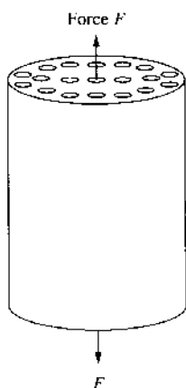
FIGURE P12.14 Unidirectional continuous-fiber reinforcement of plastics
