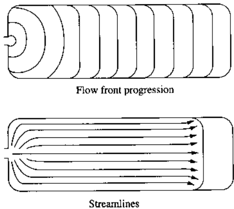
FIGURE 15.20 Mold filling under isothermal conditions. (From Ref. 28.)
