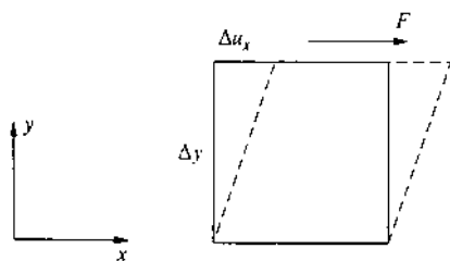
FIGURE 12.3 Shear deformation.
