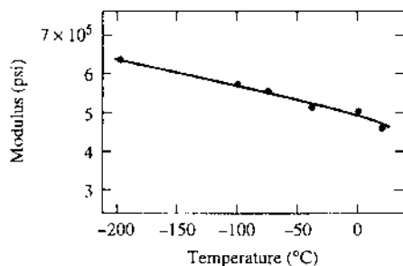
FIGURE 12.7 Effect of temperature on Young's modulus of polystyrene. (From Ref. 12.) Reprinted with permission from J. Appl. Phys., vol. 28, Rudd, J. F., and E. F. Gurnee: Photoelastic properties of polystyrene in the glassy state: II. Effect of temperature, 1096–1100, 1957. Copyright 1957 American Institute of Physics
