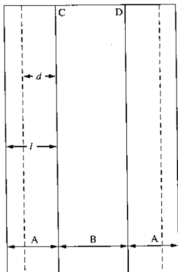
FIGURE 13.15 Diagram defining the two front penetration parameters l and d . (A), swollen region; (B), glassy region; (---), original position of surfaces; (C, D), penetrating fronts. (Reprinted from Polymer , vol. 19, Thomas N., and A. H. Windle: "Transport of Methanol in Poly(Methyl Methacrylate)," pp. 255–265, Copyright 1978, with kind permission from Elsevier Science Ltd., The Boulevard, Langford Lane, Kidlington OX5 1GB, UK.)
