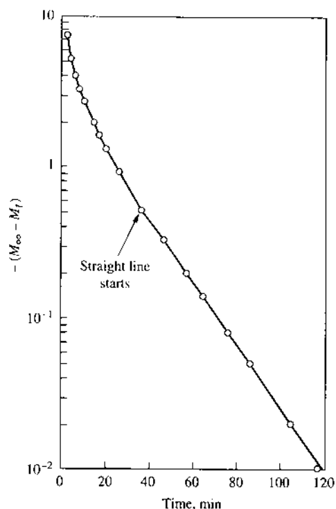
FIGURE 13.8 Typical plot for the desorption of chloroform at 25°C. (From Ref. 38.) From J. Appl. Polym. Sci., vol. 37, Saleem, M., A.-F. A. Asfour, D. DeKee, and B. Harrison: Diffusion of organic penetrants through low density polyethylene (LDPE) films: Effect of shape and size of the penetrant molecules, Copyright © 1989 by John Wiley & Sons, Inc. Reprinted by permission of John Wiley & Sons, Inc.
