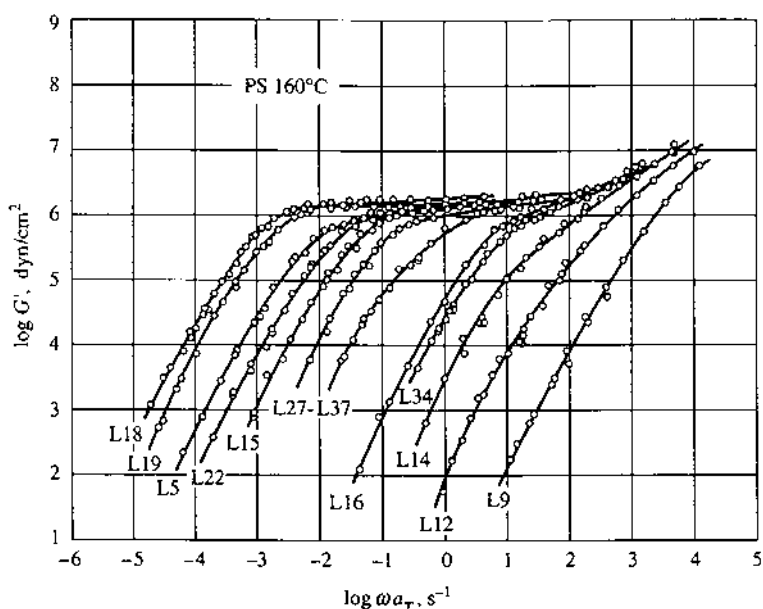
FIGURE 12.17 Master curves of G' for narrow-distribution polystyrenes having different molecular weights. The reference temperature is 160^\circ\text{C} . (Reprinted with permission from Onogi, S., T. Masuda, and K. Kitagawa: "Rheological Properties of Anionic Polystyrenes: I. Dynamic Viscoelasticity of Narrow-Distribution Polystyrenes," Macromolecules , vol. 3, pp. 109–116, 1970. Copyright 1970 American Chemical Society.)
