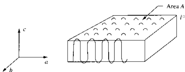
FIGURE 11.5 A chain-folded crystal lamella.
