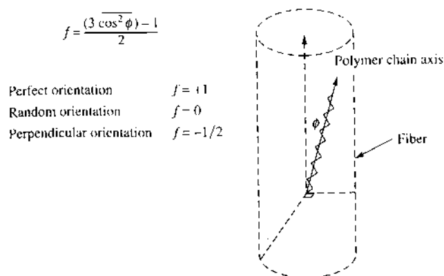
FIGURE 11.18 Schematic representation of the significance of the Hermans' orientation function. (From Ref. 58.) From Samuels, R. J.: Structured Polymer Properties . Copyright © 1974 by John Wiley & Sons, Inc. This material is used by permission of John Wiley & Sons, Inc.
