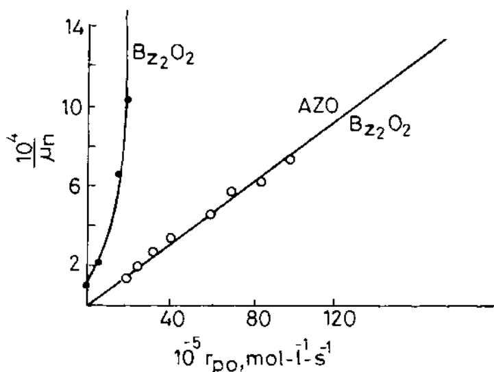
FIGURE 5.5 Average chain length ( 1/\mu_n ) versus r_{p0} at 60°C for methyl methacrylate (shown by ○) and styrene (shown by ●) for initiators azobisisobutyronitrile (AZO) and benzoyl peroxide ( Bz_2O_2 ). Rates are varied by changing initiator concentration. Data for styrene are calculated from 10^4/\mu_n = 0.6 + 12.05 \times 10^4 r_{p0} + 4.64 \times 10^8 r_{p0}^2 given in Ref. 2.
