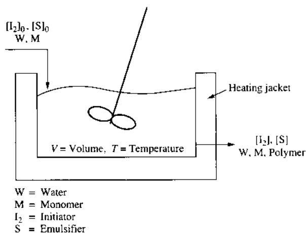
FIGURE 7.10 Schematic diagram of an HCSTR carrying out emulsion polymerization.
