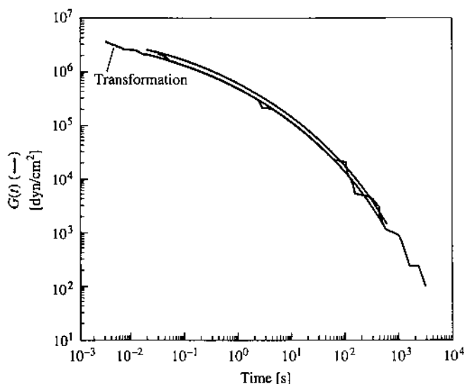
FIGURE 14.15 Stress relaxation modulus of polystyrene at 150°C.
