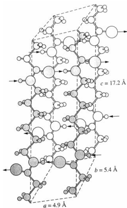
FIGURE 11.3 Perspective drawing of a unit cell of nylon 66. The viewpoint is 11 \text{ \AA} up, 10 \text{ \AA} to the right, and 40 \text{ \AA} back from the lower left corner of the cell. (From Ref. 1.)
