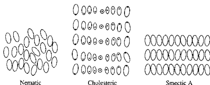
FIGURE 11.15 Schematic representation of mesophase types. (From Ref. 47.)
