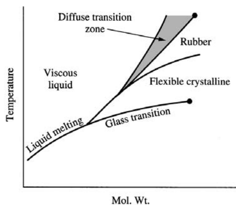
(b) Crystalline polymer
