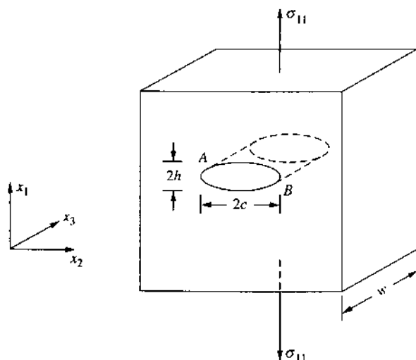
FIGURE 12.19 Crack propagation in a glassy polymer.
