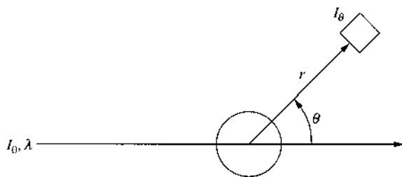
FIGURE 8.6 Schematic diagram of static light scattering.
