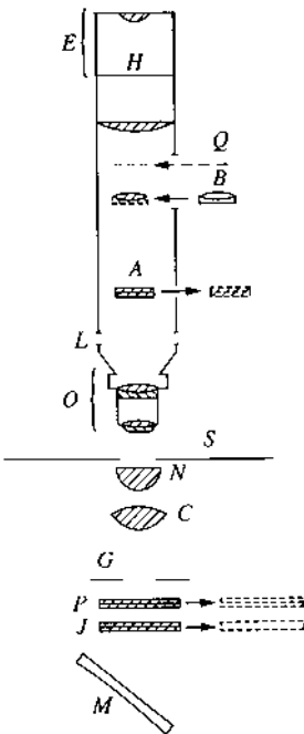
FIGURE 11.20 Arrangement of components in a typical polarizing microscope (diagrammatic).
