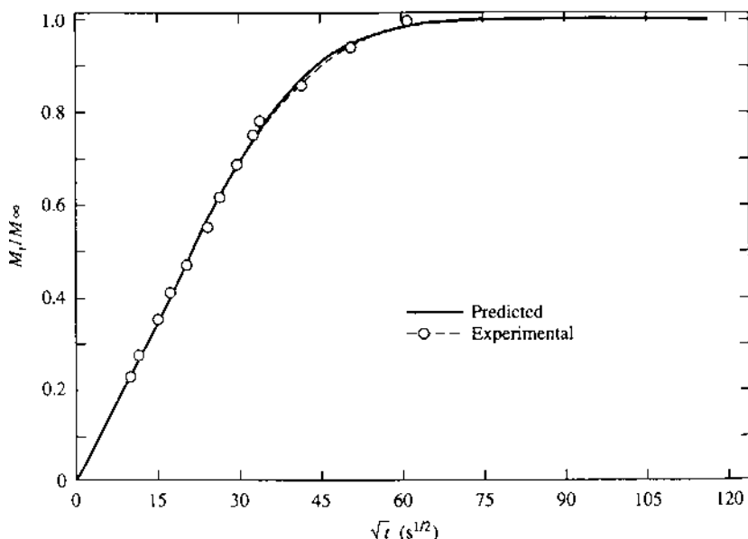
FIGURE 13.14 Fractional absorption of water vapor in Kapton ® polyimide at 30°C: membrane thickness \delta = 5 \times 10^{-3} cm (2.0 mils); pressure p = 9.55 cm Hg. (From Ref. 68). From J. Polym. Sci. Polym. Phys. Ed., vol. 27, Subramanian, S., J. C. Heydweiller, and S. A. Stern: Dual-mode sorption kinetics of gases in glassy polymers, Copyright © 1989 by John Wiley & Sons, Inc. Reprinted by permission of John Wiley & Sons, Inc.
