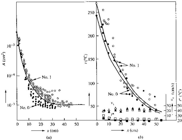
FIGURE 15.27 Filament cross section A , filament temperature t , air speed v_y , and air temperature t^* at different spinneret temperatures t_N : (○, ●) experimental; (—) theoretical. (From Ref. 54.) From J. Appl. Polym. Sci., vol. 11, Kase, S., and T. Matsuo: Studies on melt spinning: II. Steady state and transient solutions of fundamental equations compared with experimental results, Copyright © 1967 by John Wiley & Sons, Inc. Reprinted by permission of John Wiley & Sons, Inc.
