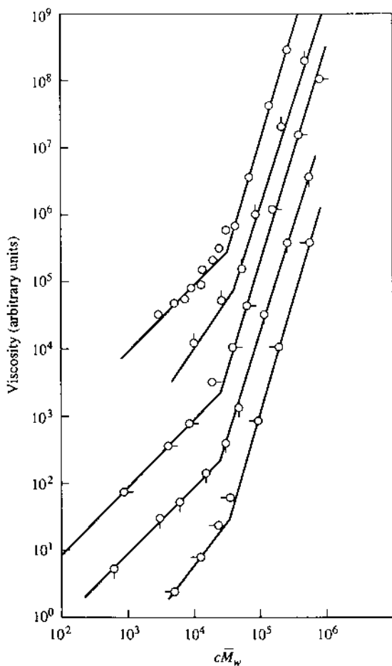
FIGURE 14.17 Viscosity versus the product c\bar{M}_w for polystyrenes at concentrations between 25% and 100%: \circ , undiluted at 217°C; \odot , 0.55 g/mL in n -butyl benzene at 25°C; \circ —, 0.415 g/mL in di-octyl phthalate at 30°C; \circ —, 0.310 g/mL in di-octyl phthalate at 30°C; and \circ —, 0.255 g/mL in n -butyl benzene at 25°C. Data at the various concentrations have been shifted vertically to avoid overlap. (From Ref. 25.) Reprinted with permission from Graessley, W. W.: The entanglement concept in polymer rheology, Adv. Polym. Sci., vol. 16, 1–179, 1974. Copyright 1974 Springer-Verlag GmbH & Co, kG.
