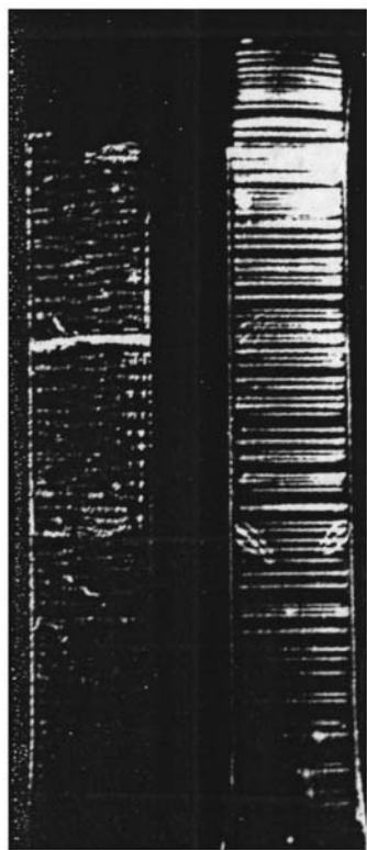
FIGURE 12.21 Craze formation in polystyrene. (From Ward, I. M., and D. W. Hadley: An Introduction to the Mechanical Properties of Solid Polymers , Wiley, Chichester, UK, 1993. Copyright John Wiley & Sons Limited. Reproduced with permission.)
