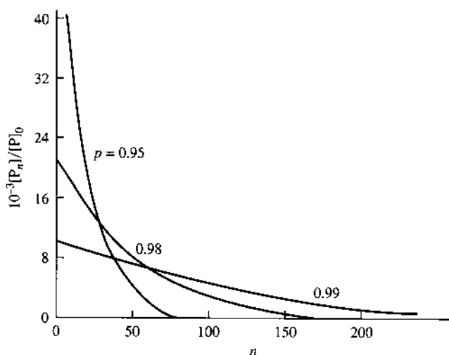
FIGURE 3.2 Number fraction distribution in ARB step-growth polymerization in batch reactors using pure monomer feed. [Reprinted from P. J. Flory, Chem. Rev., 39, vol. 137 (1946) with permission of American Chemical Society.]
