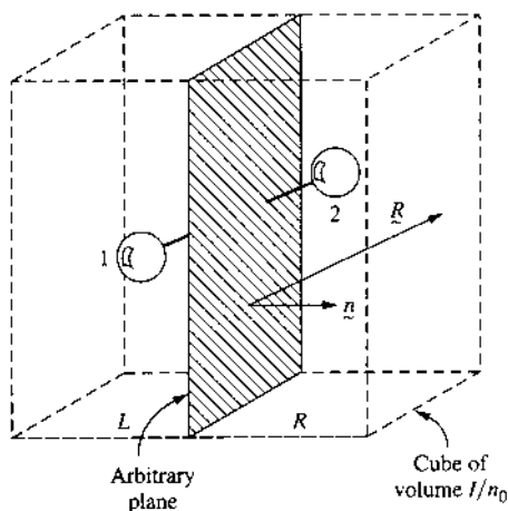
FIGURE 14.20 Calculation of the stress contributed by a dumbbell. (From Ref. 37.) Reprinted with permission from Bird, R. B., H. R. Warner, Jr., and D. C. Evans: Kinetic theory and rheology of dumbbell suspensions with Brownian motion, Adv. Polym. Sci. vol. 8, pp. 1–90. 1971. Copyright 1971 Springer-Verlag GmbH & Co. KG.
