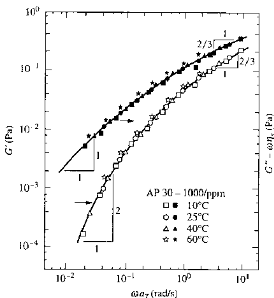
FIGURE 14.22 Master curve of G' and G'' - \omega\eta_s versus \omega a_T for 1000 ppm Separan AP30, \square, \blacksquare : 10°C; \circ, \bullet , 25°C, \triangle, \blacktriangle , 40°C, \star, \blackstar , 60°C. (From Ref. 47.) (Reprinted with permission from Tam, K. C., and C. Tiu: “Steady and Dynamic Shear Properties of Aqueous Polymer Solutions,” J. Rheol. , vol. 33, pp. 257–280, 1989.)
