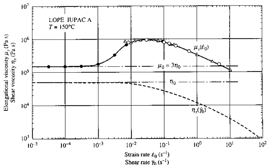
FIGURE 14.13 Steady-state viscosity in shear and elongation as a function of deformation rate. (From Ref. 14.) Reprinted from Rheol. Acta, vol. 17. Laun, H. M., and H. Munstedt: Elongational behavior of an LDPE melt: I. Strain rate and stress dependence of viscosity and recoverable strain in steady state. Comparison with shear data. Influence of interfacial tension, 415–425, 1978. Used by permission of Steinkopff Publishers, Darmstadt (FRG).
