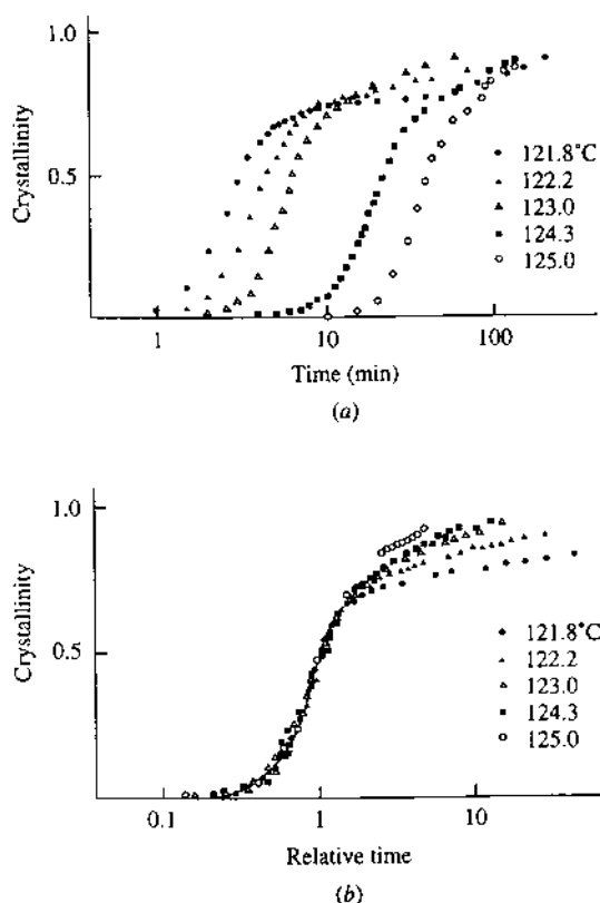
FIGURE 11.13 Isothermal crystallization data for high-density polyethylene. (a) Crystallinity-time curves in isothermal crystallization at various temperatures. (b) Plots of crystallinity versus relative time t/t^* , where t^* is time when the crystallization proceeds to 50%. (From Ref. 22.) From J. Appl. Polym. Sci., vol. 17, Nakamura, K., K. Katayama, and T. Amano: Some aspects of nonisothermal crystallization of polymers: II. Consideration of the isokinetic condition, Copyright © 1973 by John Wiley & Sons, Inc. Reprinted by permission of John Wiley & Sons, Inc.
