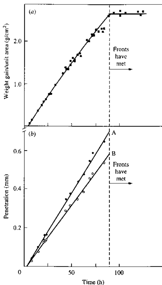
FIGURE 13.16 Data at 24^\circ\text{C} for 1-mm (nominal) sheet (actual average thickness 1.18 mm). (a) Weight gain/unit area versus time. (b) Penetration as represented by both l (A) and d (B) versus time. (Reprinted from Polymer , vol. 19, Thomas N., and A. H. Windle: "Transport of Methanol in Poly(Methyl Methacrylate)," pp. 255–265, Copyright 1978, with kind permission from Elsevier Science Ltd., The Boulevard, Langford Lane, Kidlington OX5 1GB, UK.)
