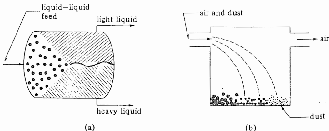
FIGURE 14.3-5. Gravity settling tanks: (a) settler for liquid-liquid dispersion, (b) dust-settling chamber.
