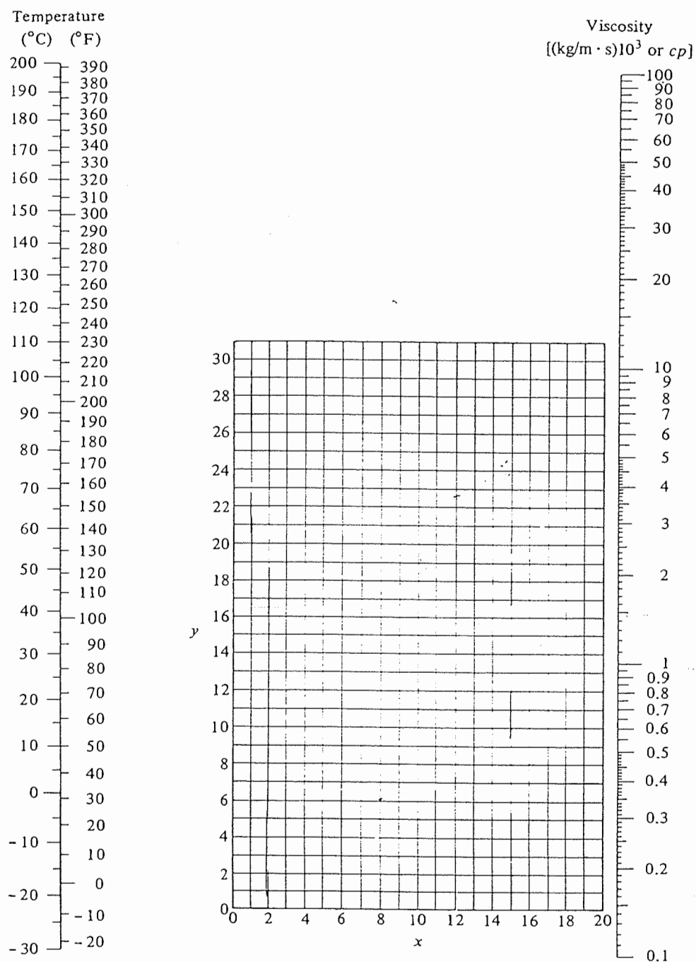
FIGURE A.3-4. Viscosities of liquids. (From R. H. Perry and C. H. Chilton, Chemical Engineers' Handbook , 5th ed. New York: McGraw-Hill Book Company, 1973. With permission.) See Table A.3-12 for use with Fig. A.3-4.
