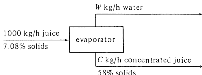
FIGURE 1.5-1. Process flow diagram for Example 1.5-1.
