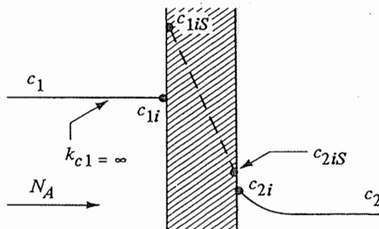
FIGURE 13.2-2. Concentrations for Example 13.2-1.
