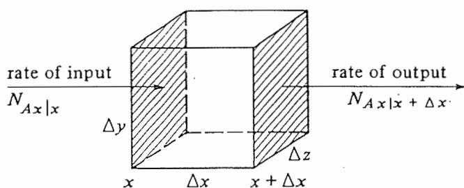
FIGURE 7.1-1. Unsteady-state diffusion in one direction.
