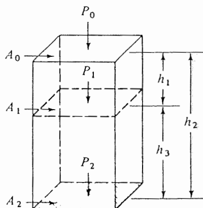
FIGURE 2.2-1. Pressure in a static fluid.
