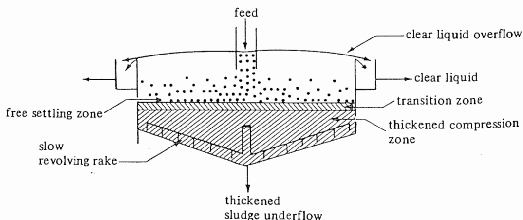
FIGURE 14.3-8. Continuous thickener.
