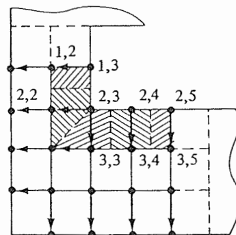
FIGURE 4.15-5. Drawing for calculation of total heat conduction.
