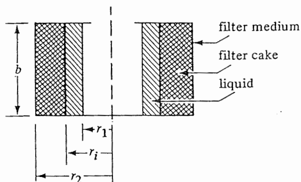
FIGURE 14.4-5. Physical arrangement for centrifugal filtration.
