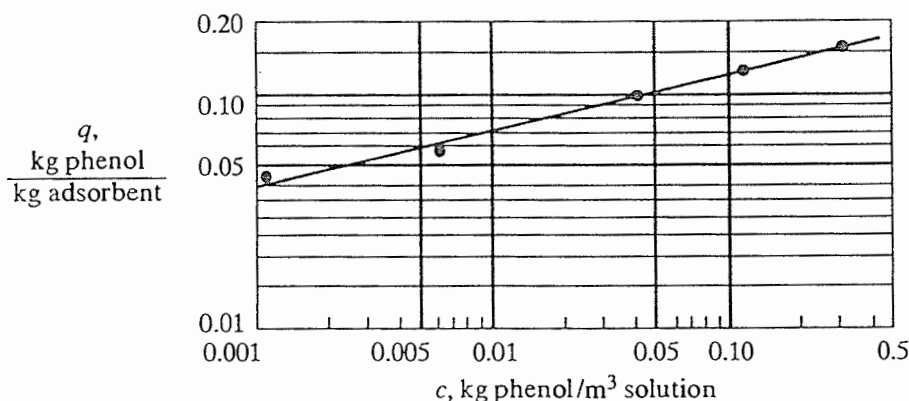
FIGURE 12.1-2. Plot of data for Example 12.1-1.
