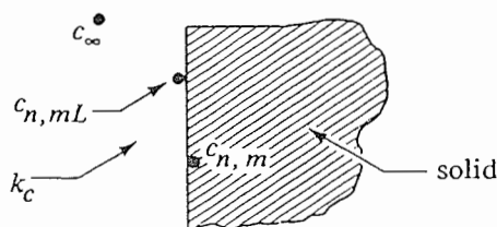
FIGURE 6.6-3. Interface concentrations for convective mass transfer at a solid surface and an equilibrium distribution coefficient K = c_{n,mL}/c_{n,m} .
