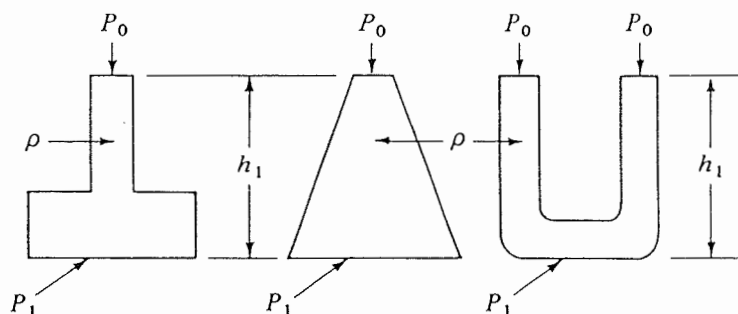
FIGURE 2.2-2. Pressure in vessels of various shapes.
