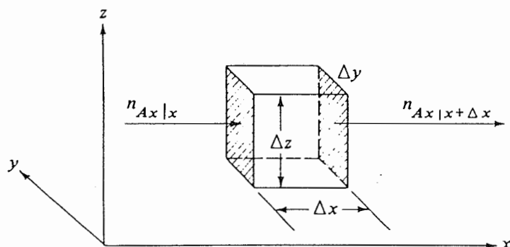
FIGURE 7.5-1. Mass balance for A in a binary mixture.
