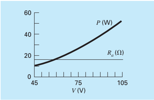
FIGURE 16.13 Results of sensitivity analysis of the effect of voltage variations on maximum power.
