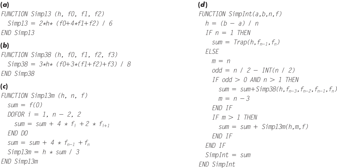
FIGURE 21.13 Pseudocode for Simpson’s rules. (a) Single-application Simpson’s 1/3 rule, (b) single-application Simpson’s 3/8 rule, (c) multiple-application Simpson’s 1/3 rule, and (d) multiple-application Simpson’s rule for both odd and even number of segments. Note that for all cases, n must be \geq 1 .
