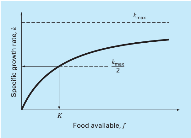
FIGURE 20.1 Plot of specific growth rate versus available food for the saturation-growth-rate model used to characterize microbial kinetics. The value K is called a half-saturation constant because it conforms to the concentration where the specific growth rate is half its maximum value.
