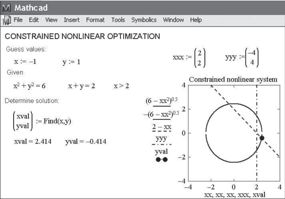
FIGURE 15.9 Mathcad screen for a nonlinear constrained optimization problem.
