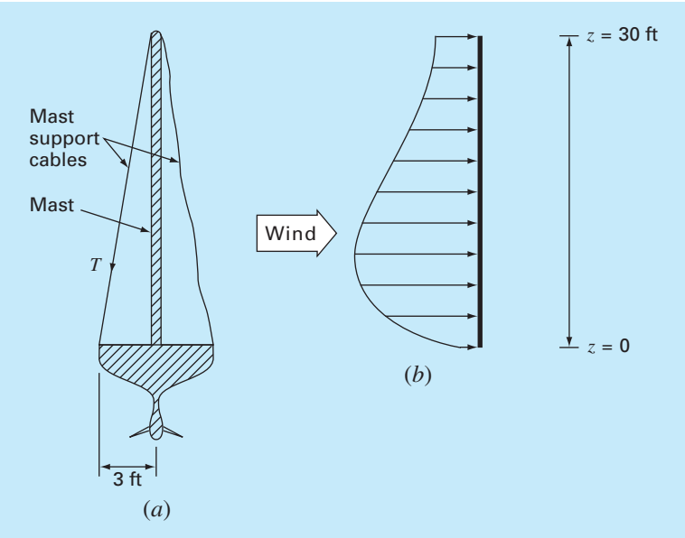
FIGURE 24.1 (a) Cross section of a racing sailboat. (b) Wind forces f exerted per foot of mast as a function of distance z above the deck of the boat.
