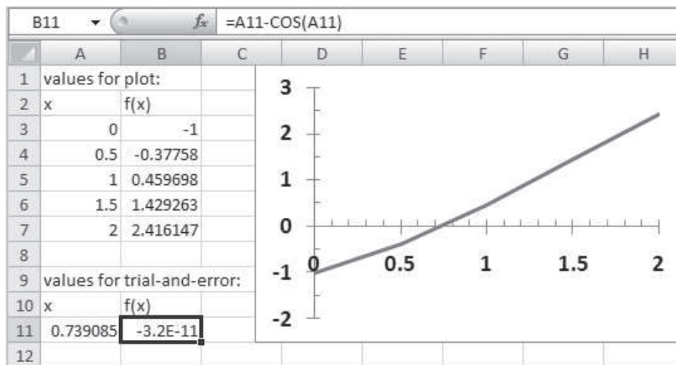
A spreadsheet set up to determine the root of f(x) = x - \cos x by trial and error. The plot is used to obtain a good initial guess.
