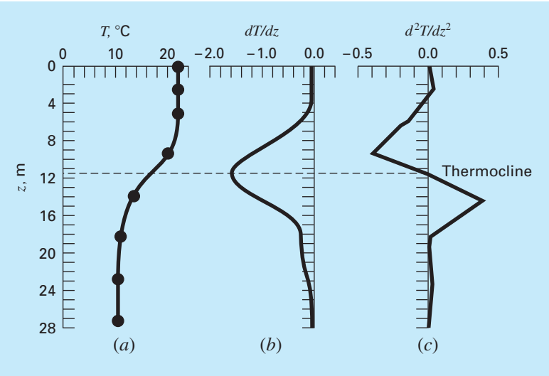
FIGURE 20.6 Plots of (a) temperature, (b) gradient, and (c) second derivative versus depth (m) generated with the cubic spline program. The thermocline is located at the inflection point of the temperature-depth curve.
