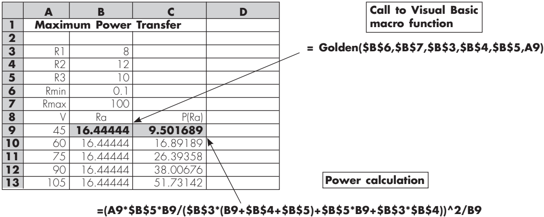
FIGURE 16.12 Excel spreadsheet to implement a sensitivity analysis of the maximum power to variations of voltage. This routine accesses the macro program for golden-section search from Fig. 16.11.
