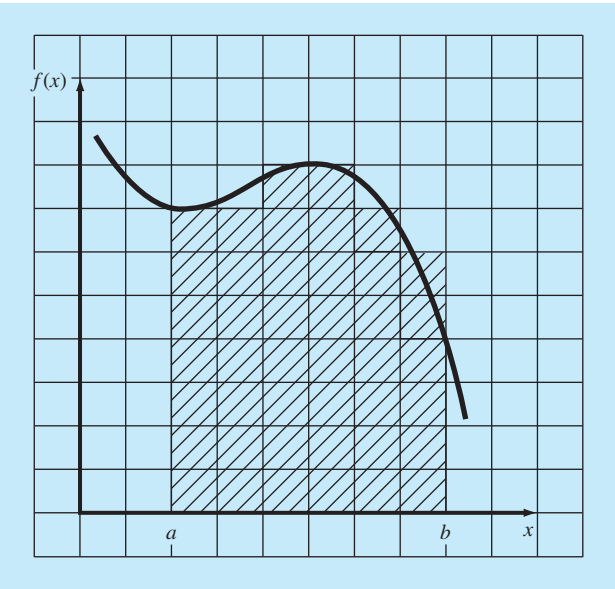
FIGURE PT6.5 The use of a grid to approximate an integral.
