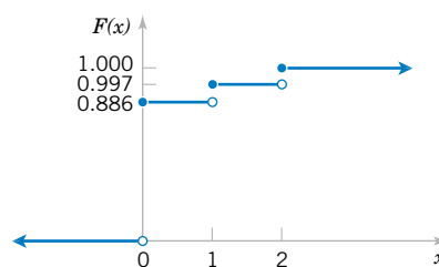
Figure 3-4 Cumulative distribution function for Example 3-8.
