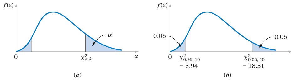
Figure 8-9 Percentage point of the \chi^2 distribution. (a) The percentage point \chi^2_{\alpha,k} . (b) The upper percentage point \chi^2_{0.05,10} = 18.31 and the lower percentage point \chi^2_{0.95,10} = 3.94 .
