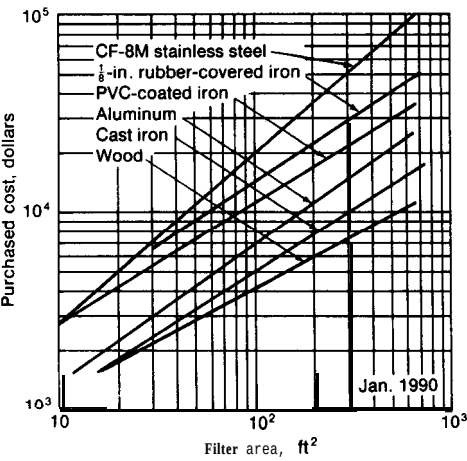
FIGURE 14-65 Plate-and-frame filters. Order-of-magnitude capital-cost estimating data.
