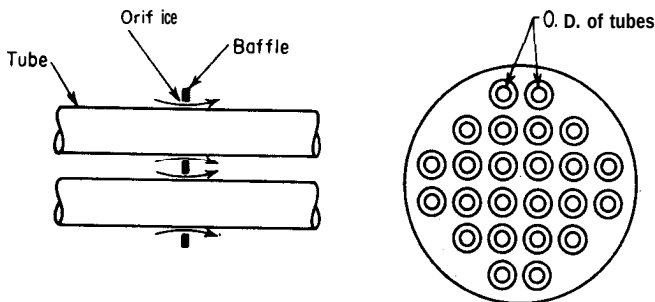
FIGURE 15-11 Orifice baffles.
