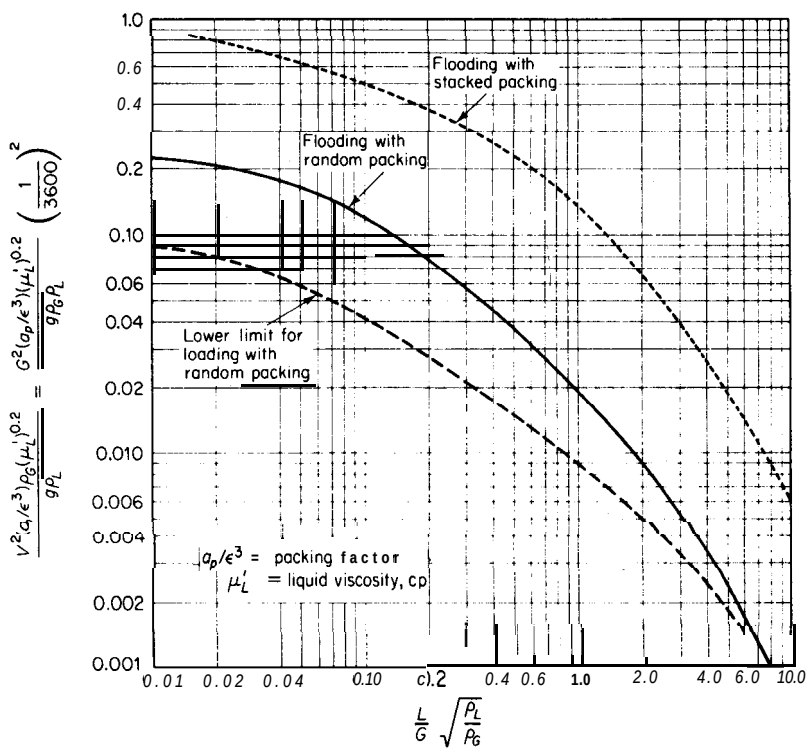
FIGURE 16-20 Correlation for estimating flooding rate in packed towers.
