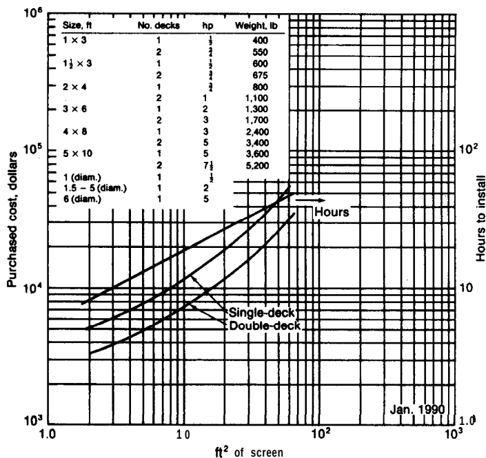
FIGURE 14-88 Vibrating screens.
