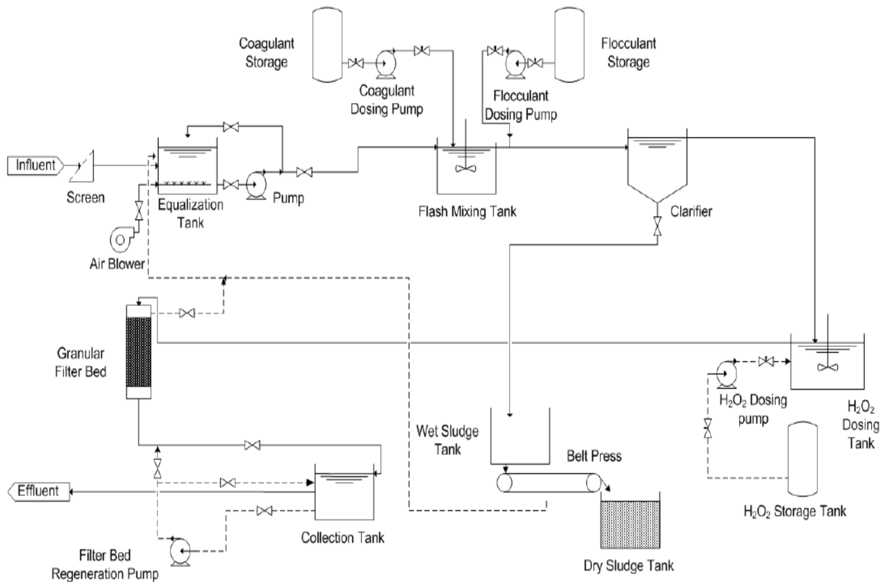
Figure 1: PFD of physico-chemical treatment of paper mill effluent (raw material: imported pulp/recycled paper)
