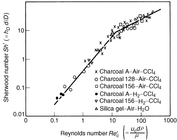
Figure 6.27. Sherwood number as a function of Reynolds number for adsorption experiments (115)
