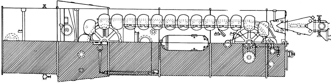
Figure 10.2. Bollmann extractor
