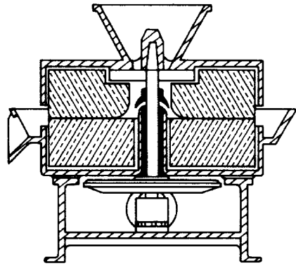
Figure 2.18. Buhrstone mill
