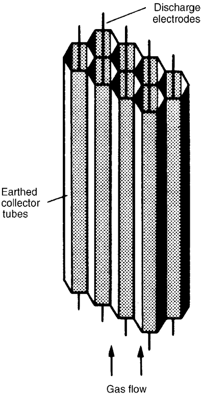
Figure 1.64. General arrangement of wire-in-tube precipitator
