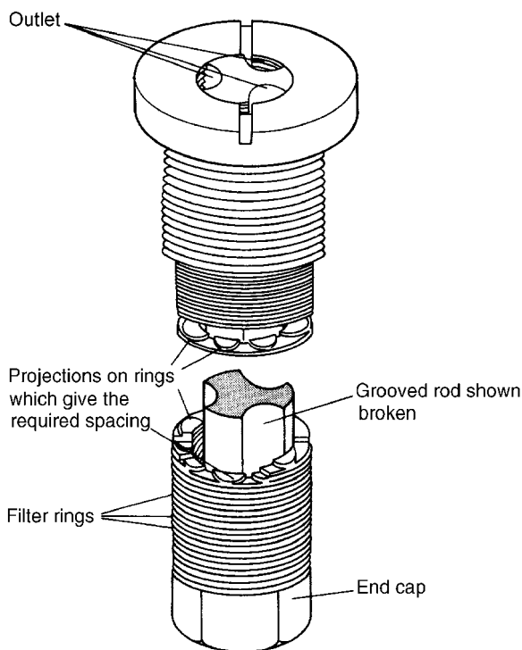
Figure 7.14. Metafilter pack (Stella Meta)
