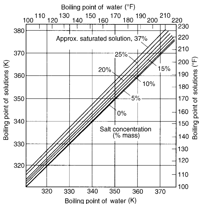
Figure 14.1. Boiling point of solutions of sodium chloride as a function of the boiling point of water. Dühring lines
