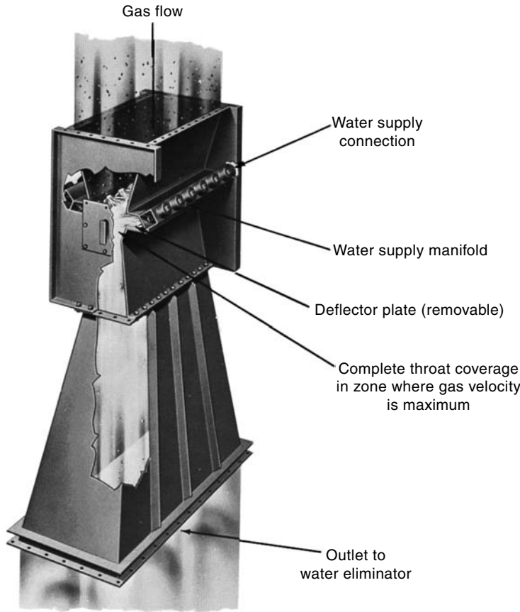
Figure 1.70. The AAF KINPACTOR venturi scrubber
