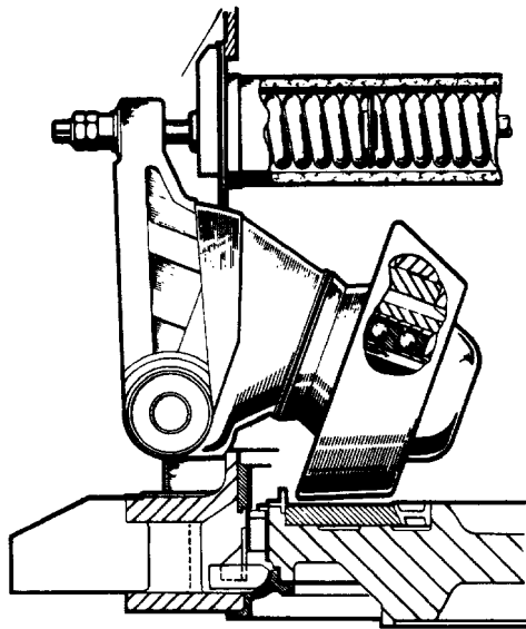
Figure 2.20. Crushing roller in a Lopulco mill
