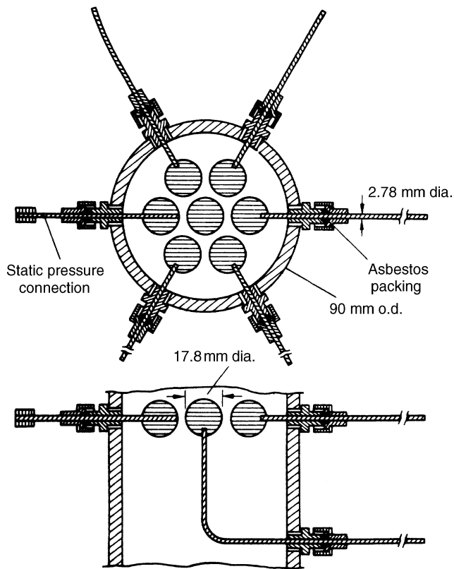
Figure 5.21. Arrangement of hexagonal spacing of particles in tube (66)
