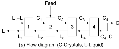
(a) Flow diagram (C-Crystals, L-Liquid)
