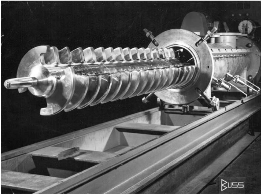
Figure 1.24. The Buss kneader
