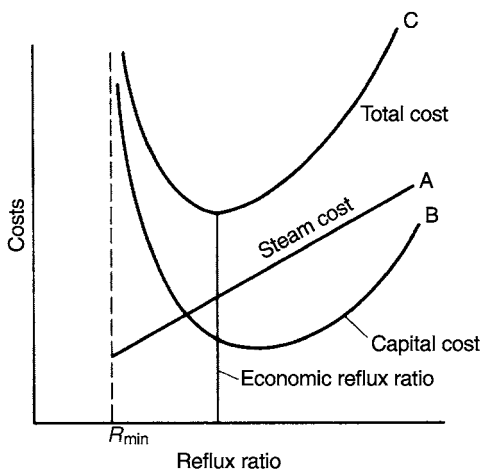
Figure 11.19. Influence of reflux ratio on capital and operating costs of a still
