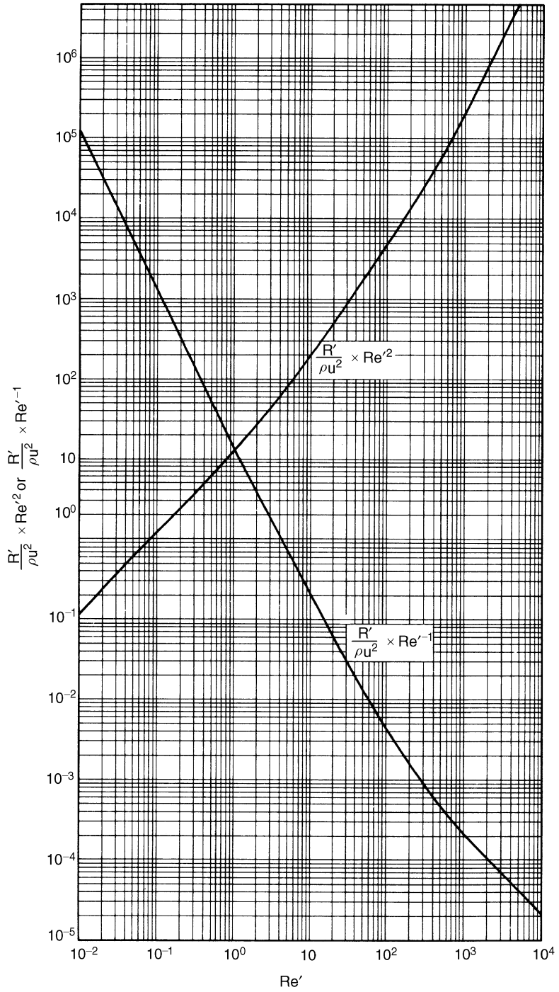
Figure 3.6. (R'/\rho u^2)Re'^2 and (R'/\rho u^2)Re'^{-1} versus Re' for spherical particles
