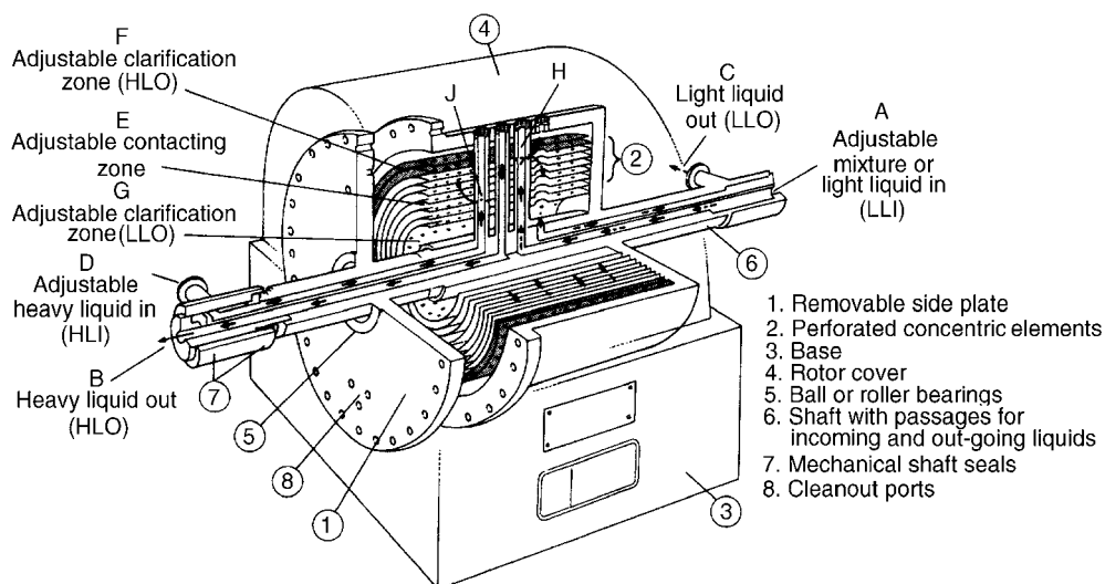
Figure 13.39. Podbielniak contactor
