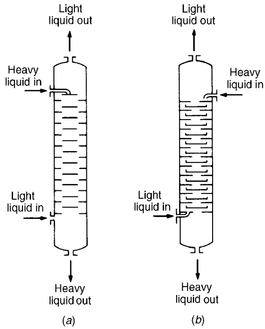
Figure 13.29. Baffle-plate column
