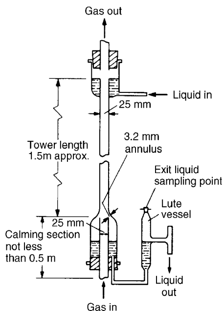
Figure 12.3. Diagram of a typical laboratory wetted-wall column
