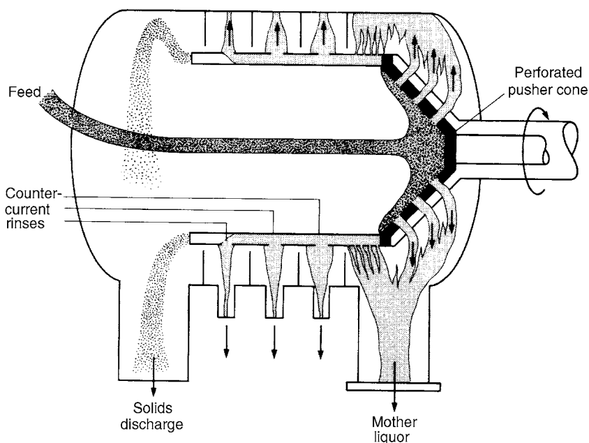
Figure 9.16. Pusher-type centrifuge
