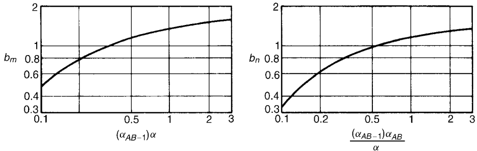
Figure 11.41. Factors in Colburn's solution
