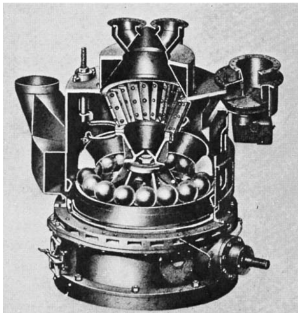
Figure 2.19. Babcock mill
