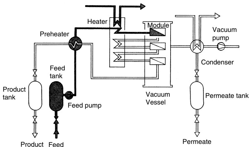
Figure 8.20. Schematic diagram of a pervaporation unit
