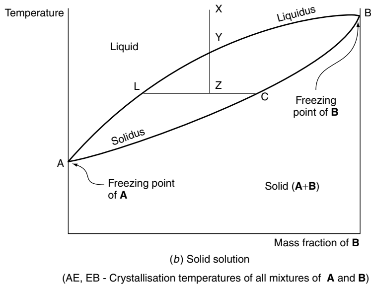
Figure 15.3. Phase diagrams for binary systems
