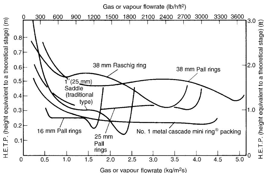
Figure 11.59. Height equivalent to a theoretical stage for common packings
