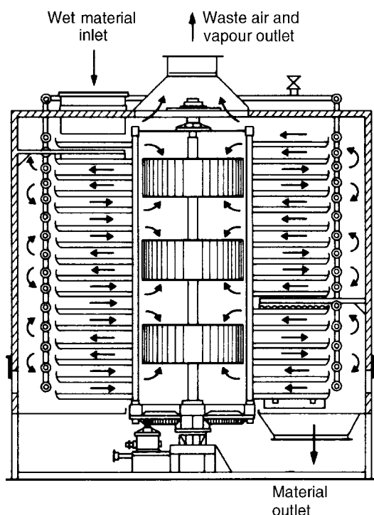
Figure 16.30. Turbo-shelf dryer
