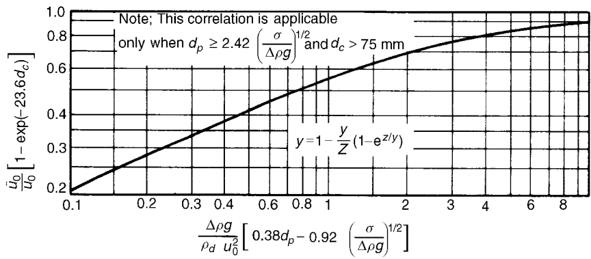
Figure 13.37. Chart for calculation of velocity ( \bar{u}_0 ) of a single droplet relative to continuous phase ( d_c and d_p are in m) (27)
