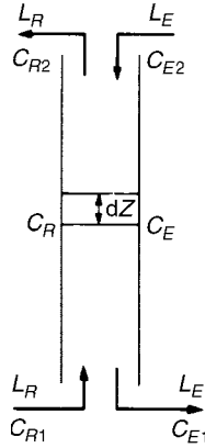
Figure 13.20. Countercurrent flow in a packed column
