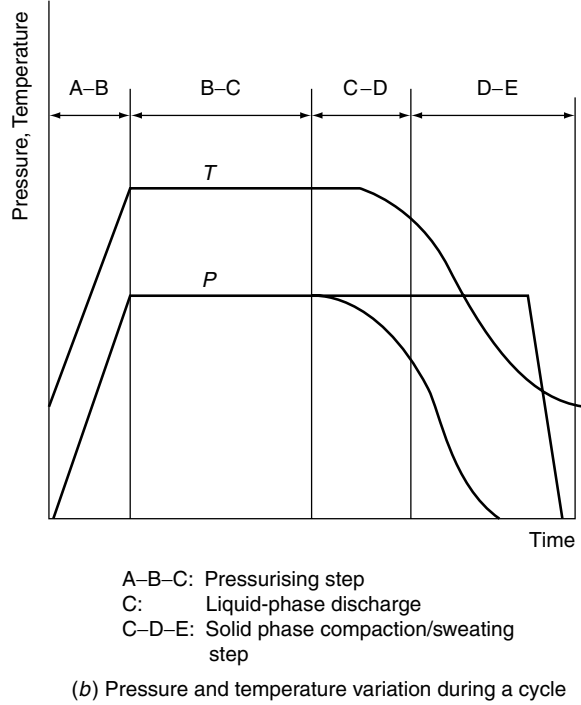
Figure 15.38. High pressure crystallisation
