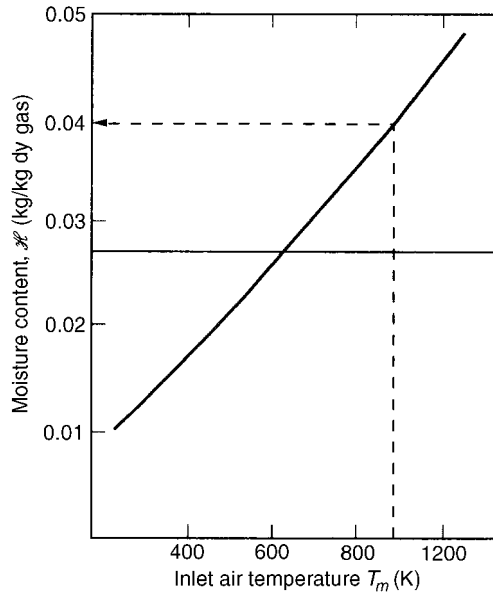
Figure 16.28. Moisture content of the inlet air (47)
