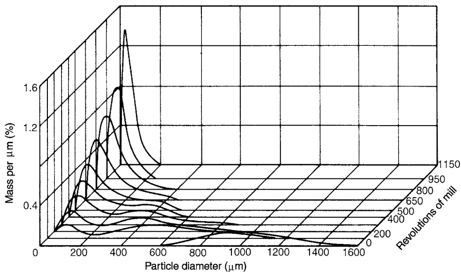
Figure 2.1. Effect of progressive grinding on size distribution
