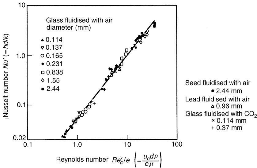
Figure 6.30. Correlation of experimental results for heat transfer to particles in a fluidised bed (121)
