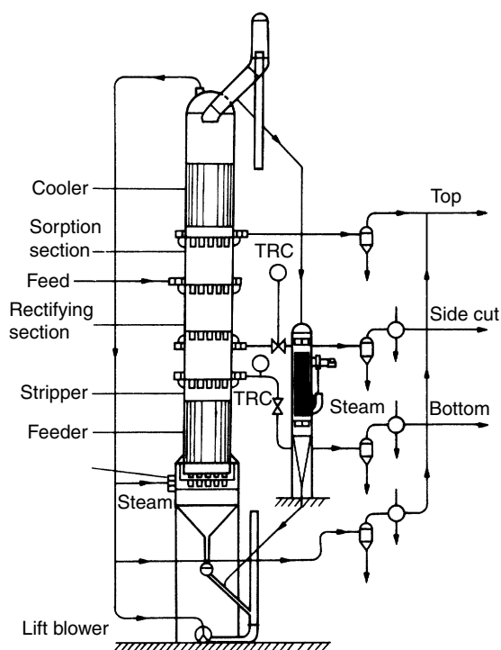
Figure 17.26. The hypersorber (45)
