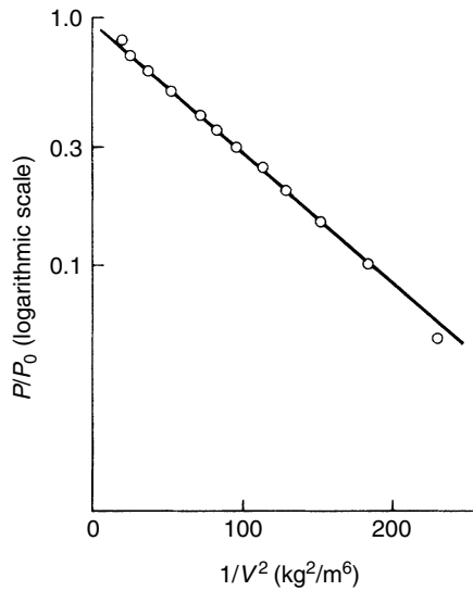
Figure 17.14. Harkins-Jura plot for Example 17.2
