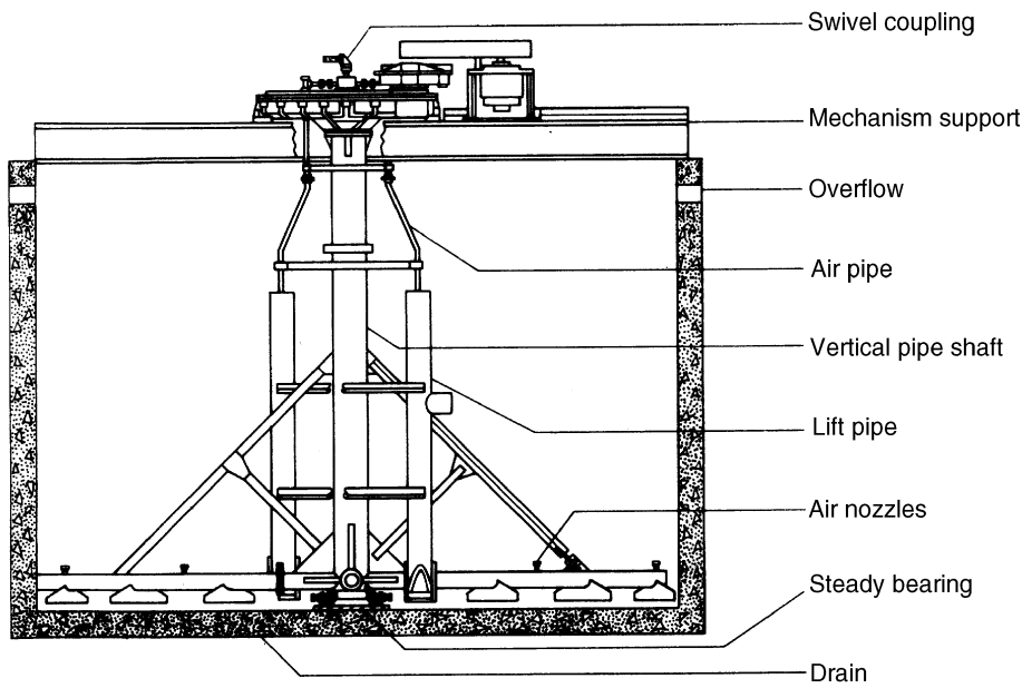
Figure 10.9. Dorr agitator
