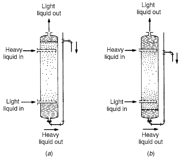
Figure 13.32. Spray towers
