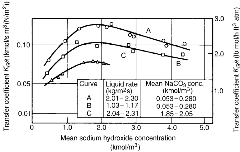
Figure 12.13. Absorption of carbon dioxide in sodium hydroxide solution G' = 0.24\text{--}0.25 kg/m 2 s, temperature = 298 K
