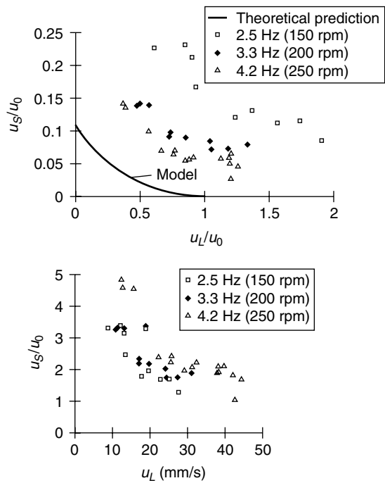
Figure 20.16. Experimental flooding data for the ion-exchange resin ( d = 190\text{ }\mu\text{m} , \rho_s = 1,250\text{ kg/m}^3 ) in the low- g rotor with backflow of the solids discharge (20)
