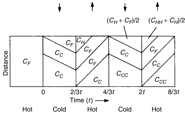
Figure 17.36. Effect of cycle-time on separation
