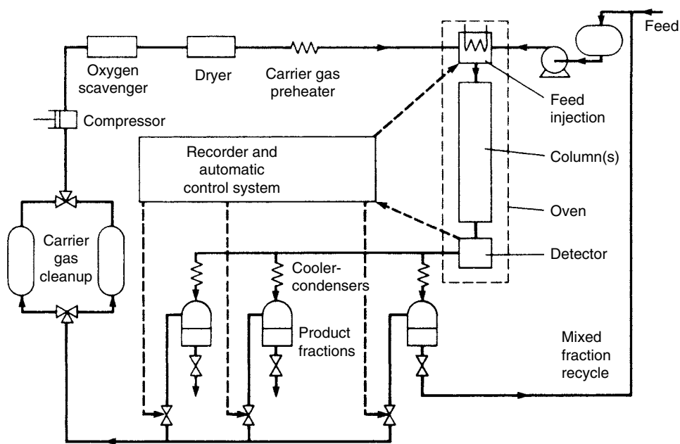
Figure 19.5. Production gas-chromatograph
