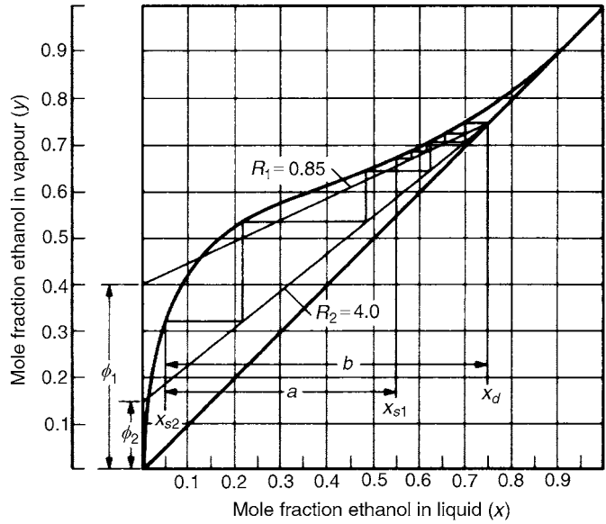
Figure 11.35. Batch distillation—constant product composition
