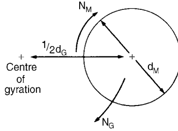
Figure 2.32. Geometry of the planetary mill
