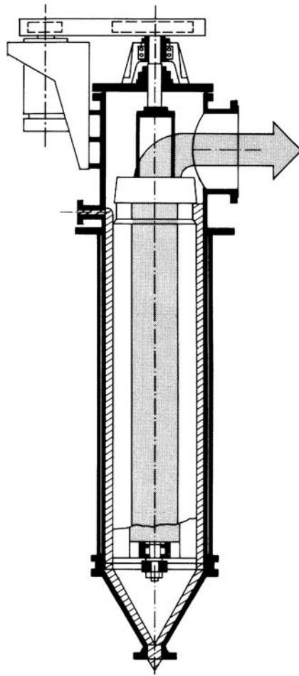
Figure 14.24. Thin-film evaporator
