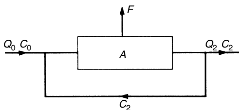
Figure 8.15. Single 'feed and bleed' stage
