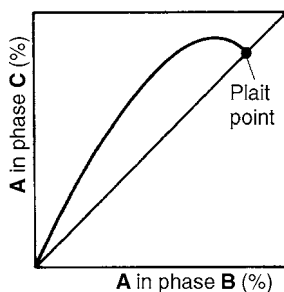
Figure 13.8. Equilibrium distribution of solute A in phases B and C
