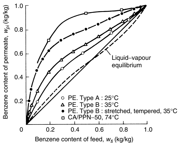
Figure 8.21. Comparison of selectivity of pervaporation membranes and liquid-vapour equilibrium for benzene/cyclohexane mixtures
