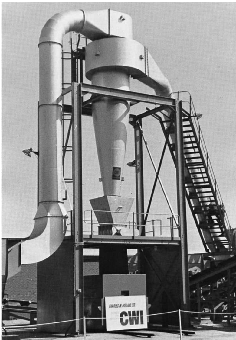
Figure 1.54. Cyclone separator
