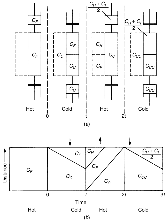
Figure 17.35. Ideal parapump, direct heating (a) Dotted section represents the condition immediately after a temperature change but before the pistons move (b) Position of the wave-front against time
