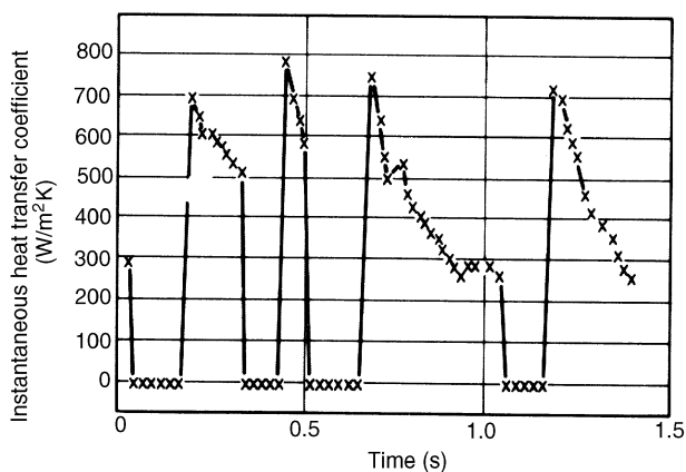
Figure 6.24. Instantaneous heat transfer coefficients for glass beads fluidised in air (110)
