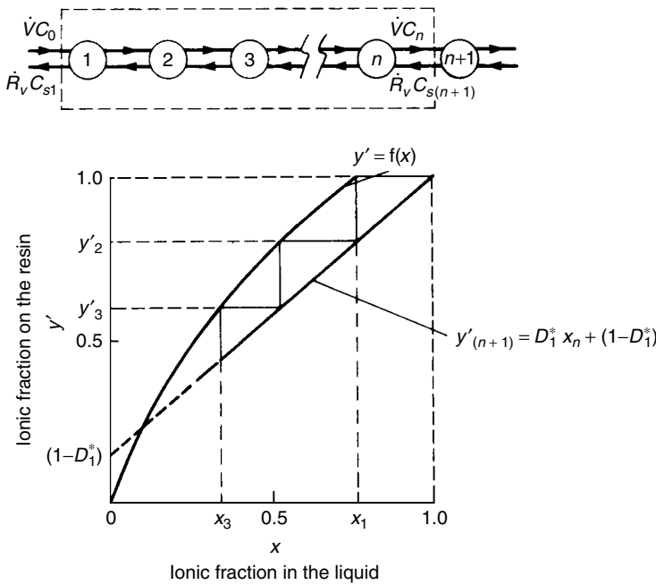
Figure 18.6. Multistage countercurrent ion-exchange
