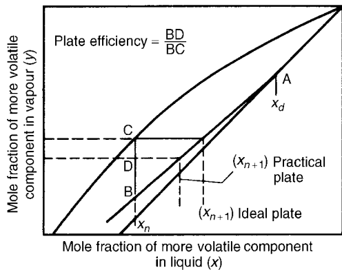
Figure 11.56. Graphical representation of plate efficiency E_{Mr}
