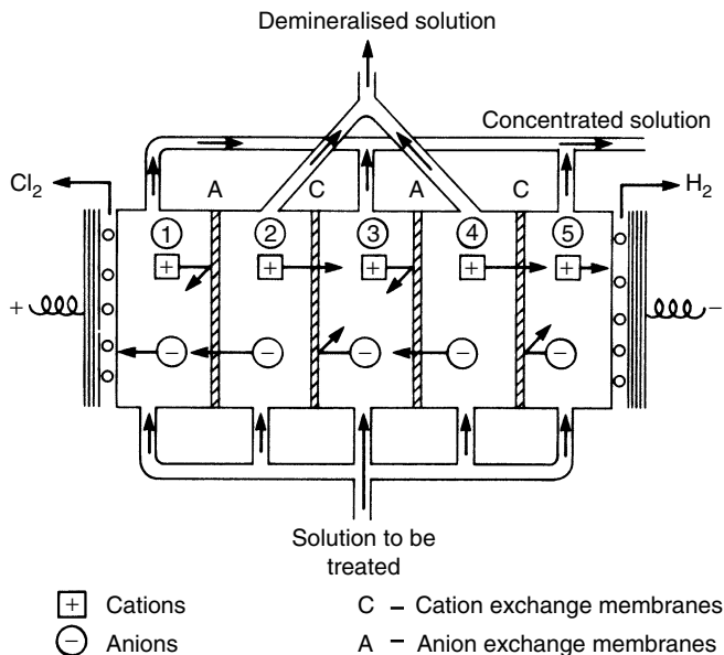
Figure 8.17. Schematic flow-diagram for an electrodialysis stack
