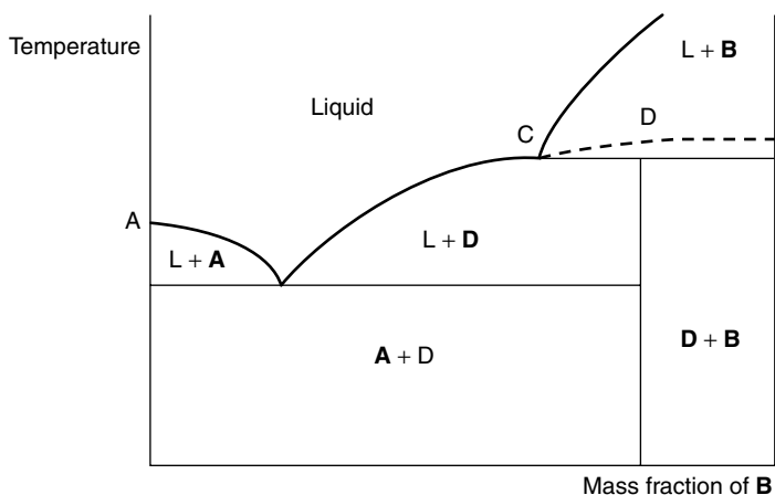
(b) Incongruent melting point
