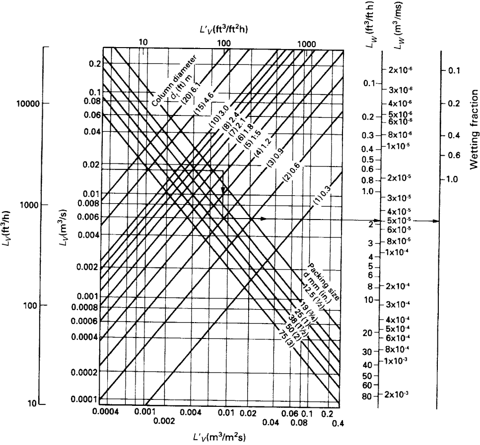
Figure 4.19. Nomograph for the estimation of the degree of wetting in a packed column (49)
