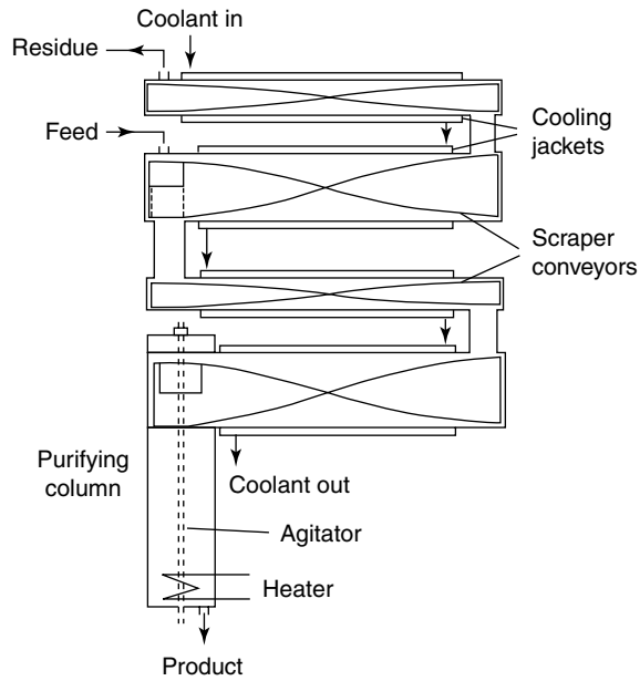
Figure 15.28. Brodie purifier (89)
