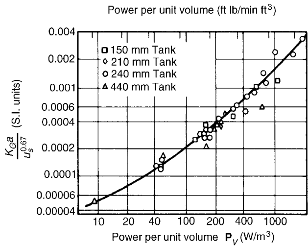
Figure 12.30. General correlation of data for a vessel (height = diameter) with vaned-disc agitator
