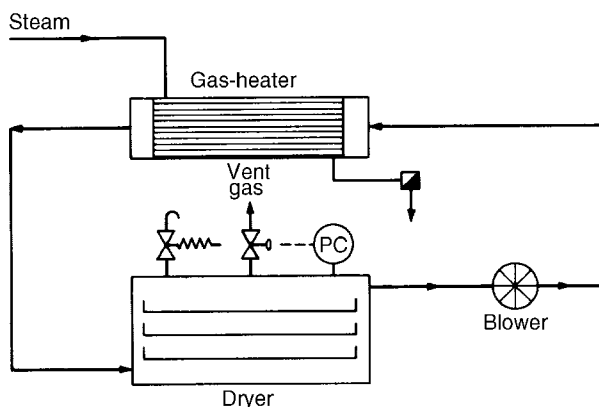
Figure 16.33. Superheated-steam dryer
