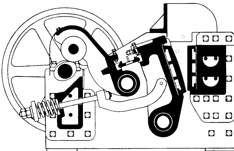
Figure 2.5. Dodge crusher
