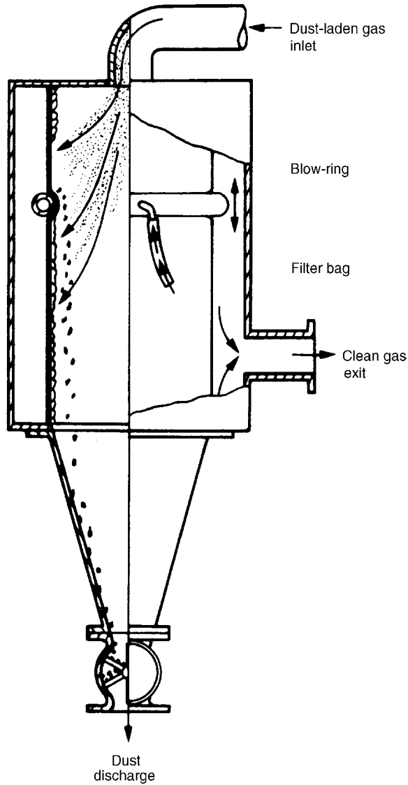
Figure 1.61. Reverse-jet filter (52)
