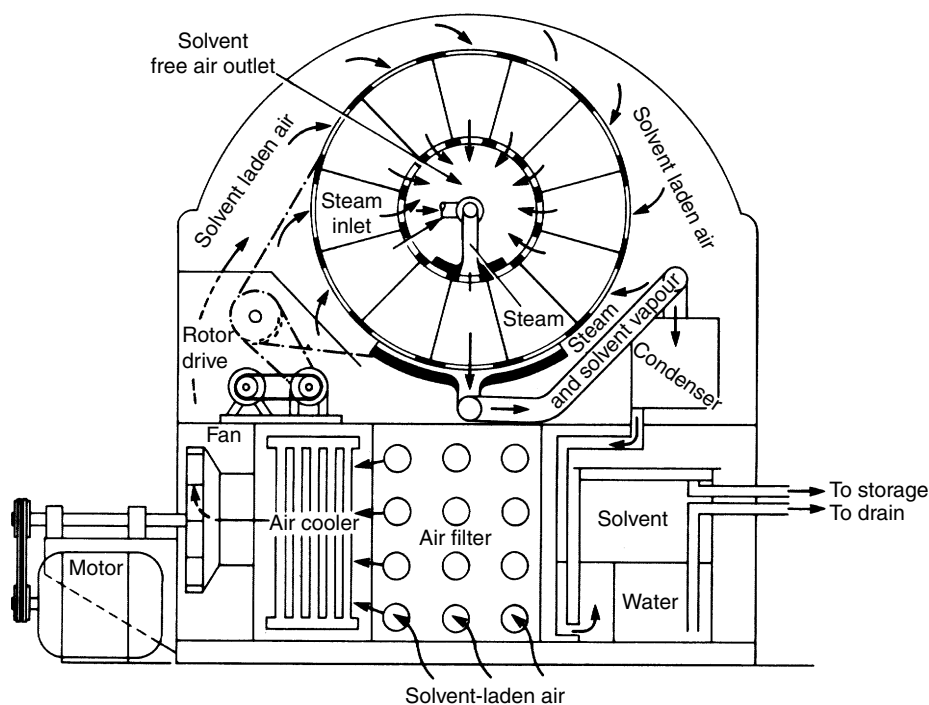
Figure 17.29. Rotary-bed adsorber
