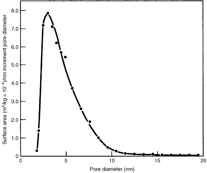
Figure 17.12. Pore size distribution of an activated alumina calculated from the isotherm by the method of Cranston and Inkley (26)
